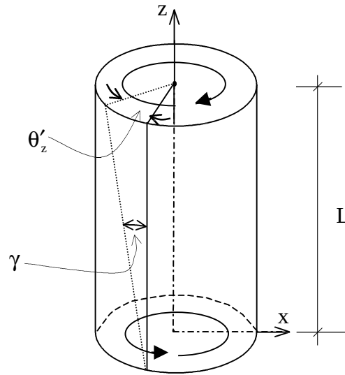
Figure 3.10. Twisting of a circular shaft (no warping)
