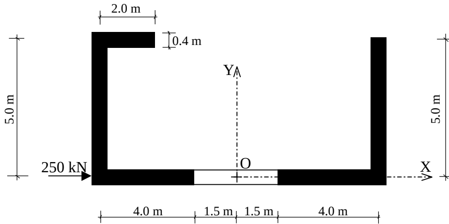
Figure 6.57. Cross-sectional view of the structure in Example 16
