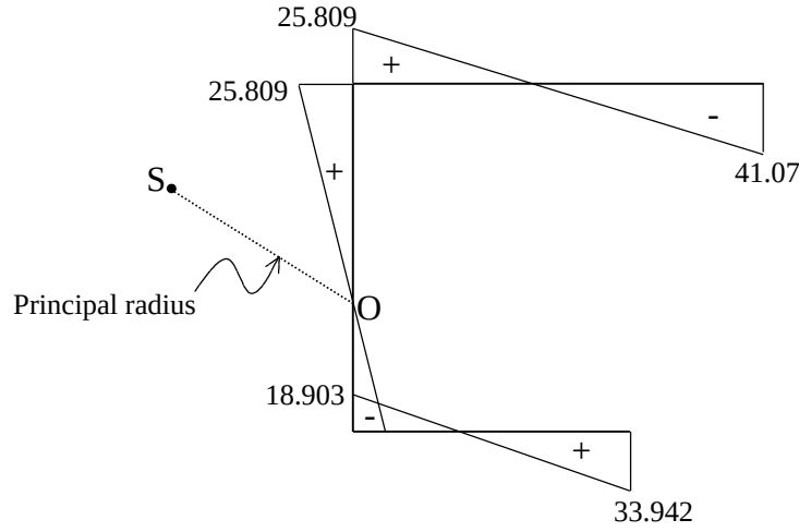
Figure A4.4. Principal sectorial area diagram
