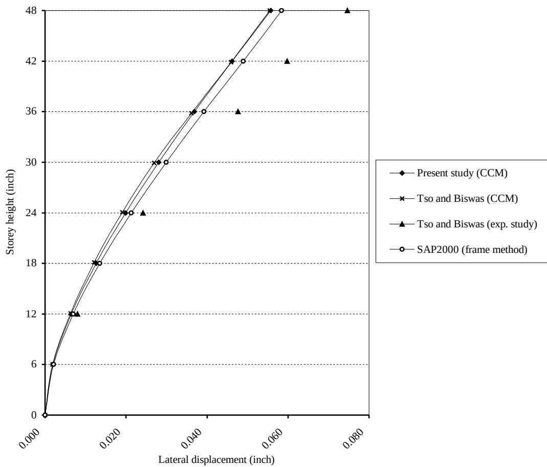
Figure 6.2. The lateral displacements in the X direction in Example 1
