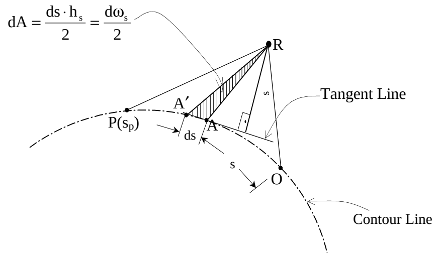
Figure 3.5. Computation of sectorial area
