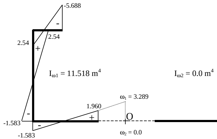
Figure 6.23. The principal sectorial area diagram of the structure in Example 7
