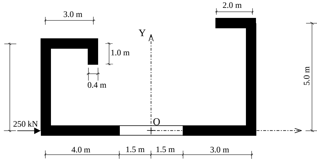
Figure 6.25. Cross-sectional view of the structure in Example 8
