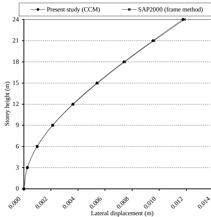
Figure 6.20. The lateral displacements in the Y direction in Example 6
