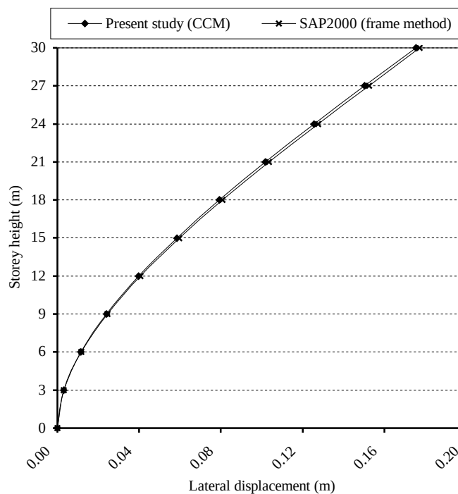
Figure 6.30. The lateral displacements in the X direction in Example 9
