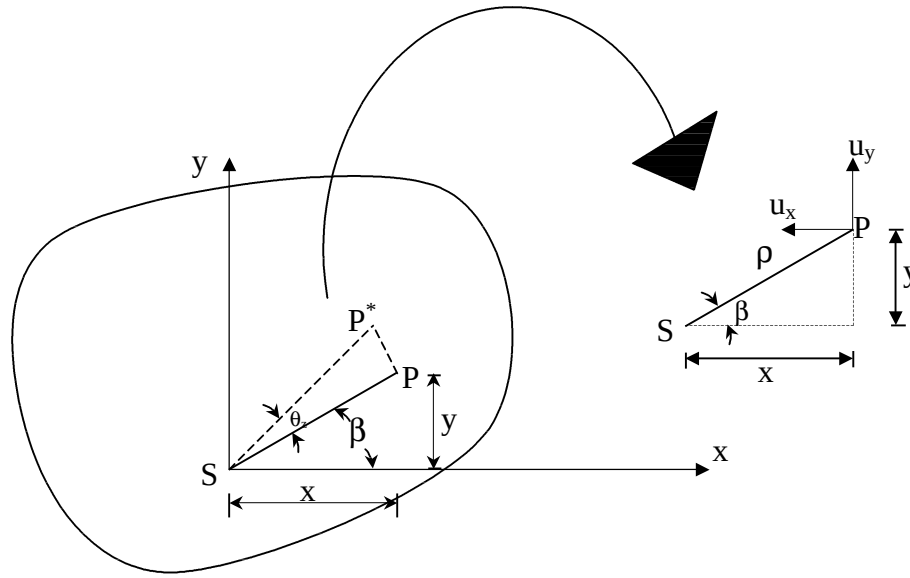
Figure 3.20. Displacements of a non-circular bar due to rotation
