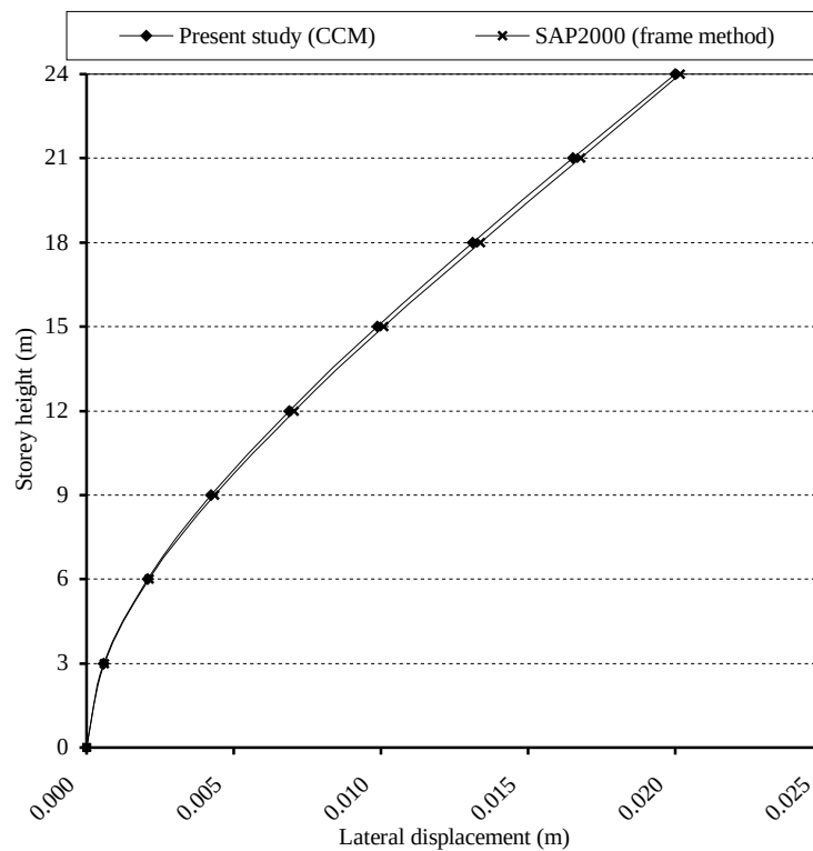
Figure 6.19. The lateral displacements in the X direction in Example 6
