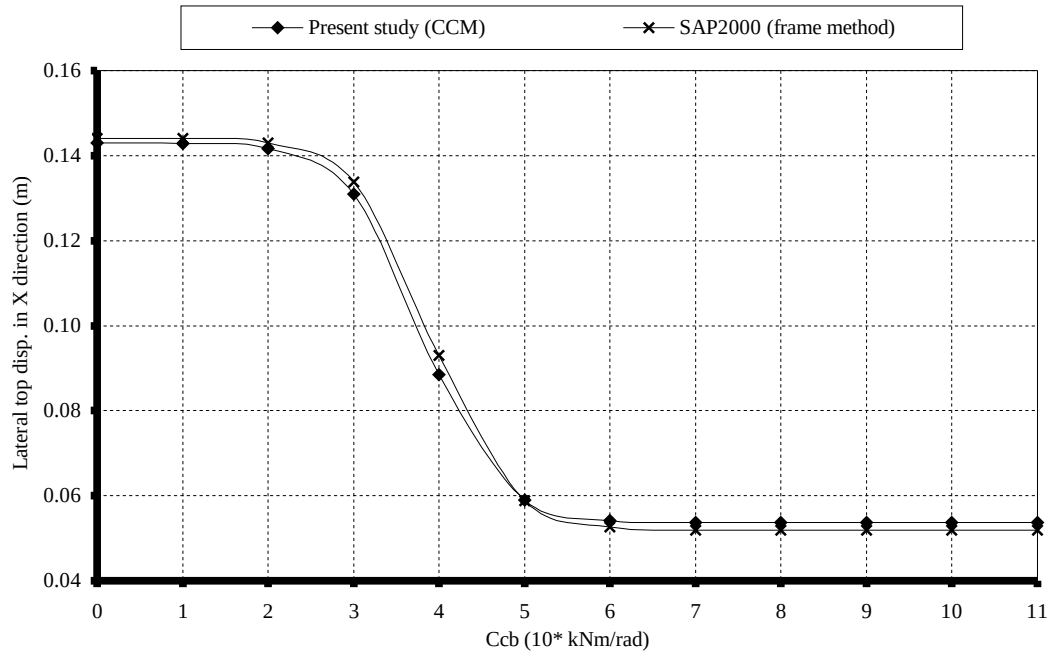
Figure 6.54. The effect of the variation of the connection stiffness on the maximum top displacement in the X direction in Example 15
