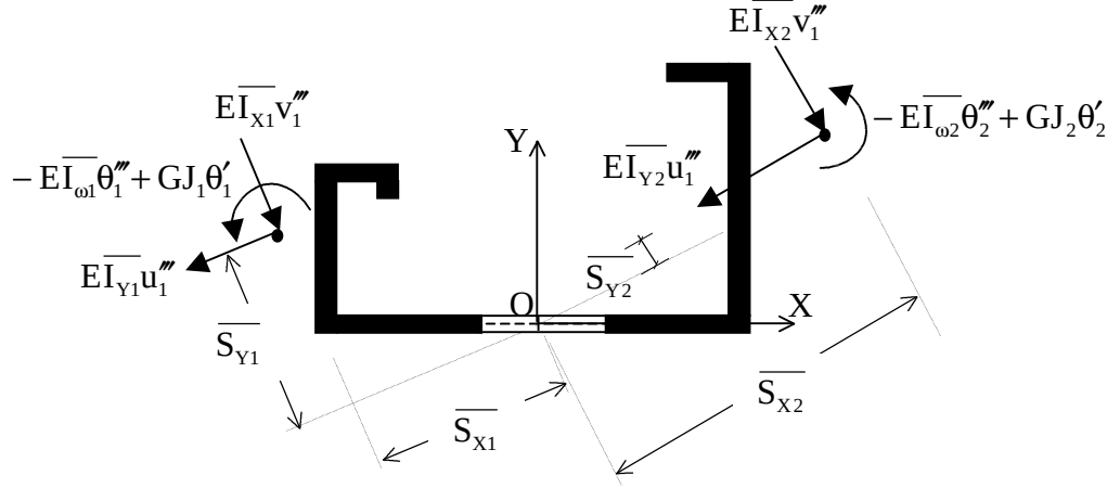
Figure 5.12. Internal torques and shear forces
