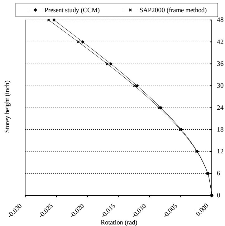
Figure 6.12. The rotations about the Z direction in Example 4
