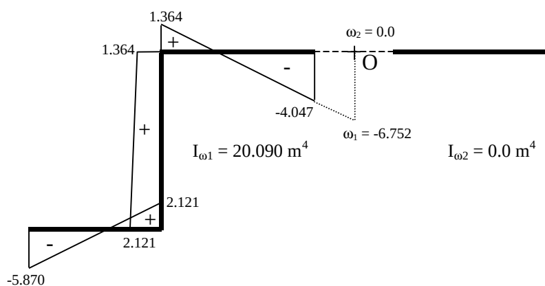
Figure 6.18. The principal sectorial area diagram of the structure in Example 6
