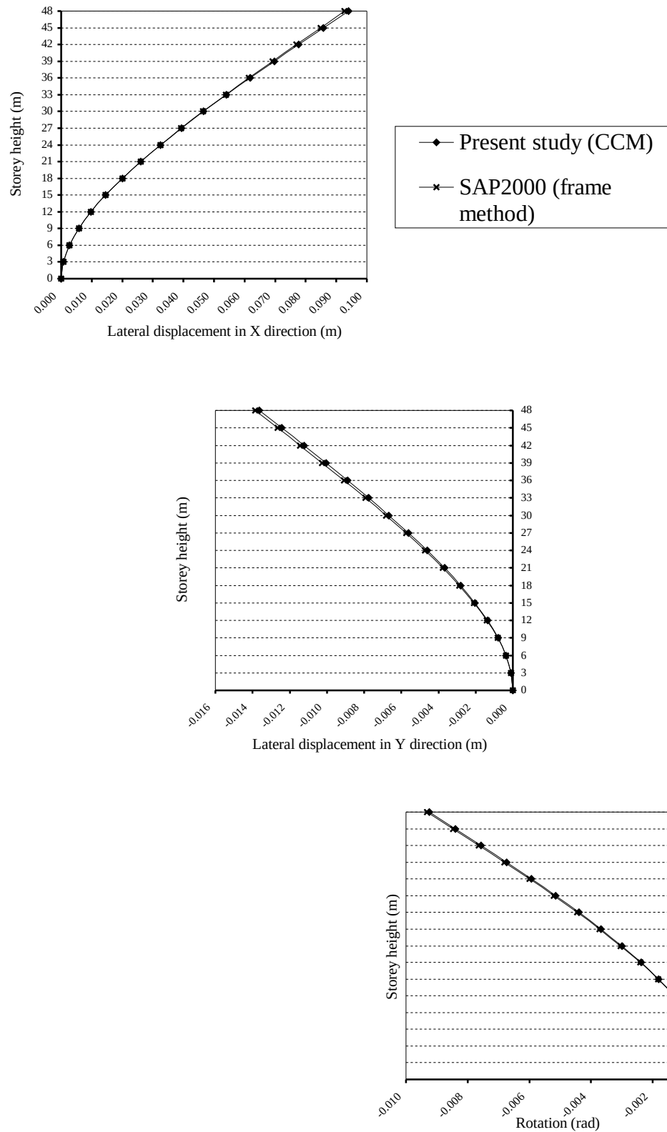
Figure 6.24. The lateral displacements and the rotations along the height in Example 7
