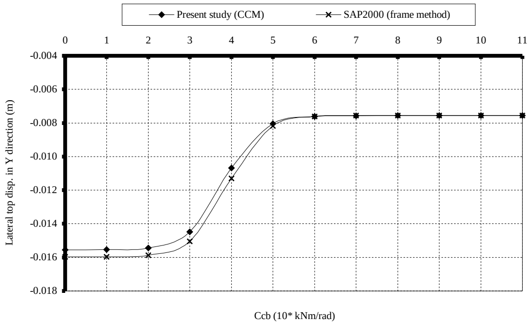
Figure 6.55. The effect of the variation of the connection stiffness on the maximum top displacement in the Y direction in Example 15
