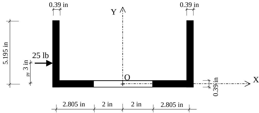
Figure 6.10. Cross-sectional view of the structure in Example 4
