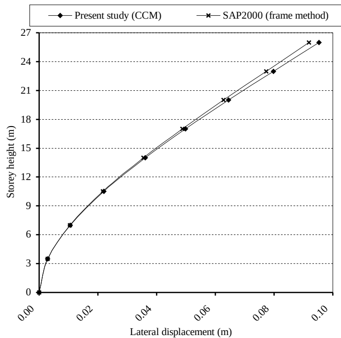
Figure 6.44. The lateral displacements in the X direction in Example 12
