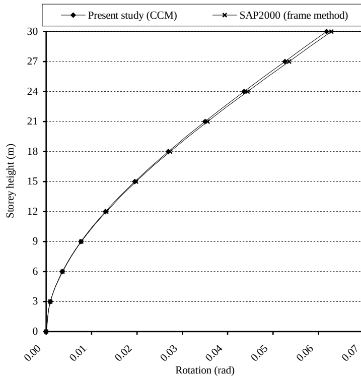
Figure 6.37. The rotations about the Z direction in Example 10
