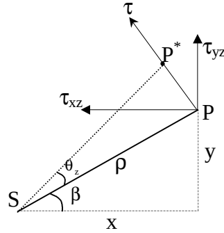
Figure 3.18. Shear stresses in uniform torsion
