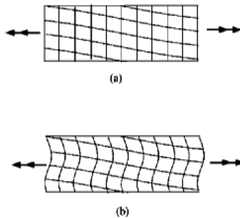
Figure 3.19. (a) Torsion of a circular bar with no out-of-plane warping (b) Torsion of a non-circular bar with warping
