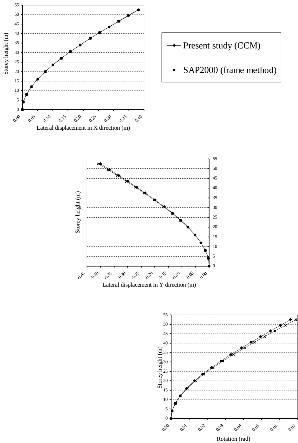
Figure 6.52. The lateral displacements and the rotations along the height in Example14
