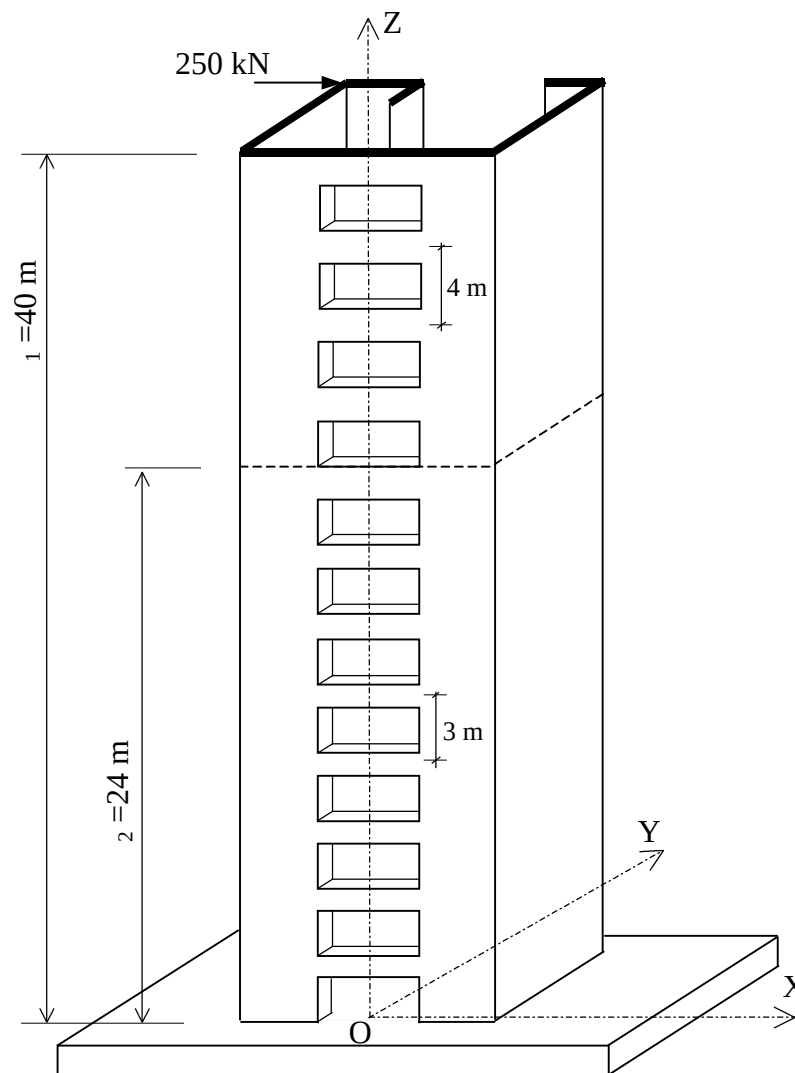
Figure 6.46. Geometrical properties and loading of the structure in Example 13
