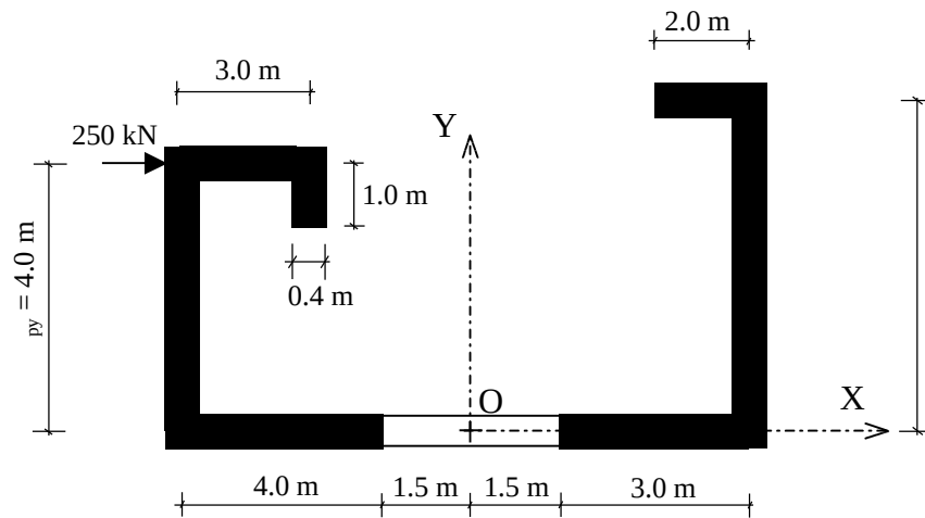
Figure 6.47. Cross-sectional view of the structure in Example 13
