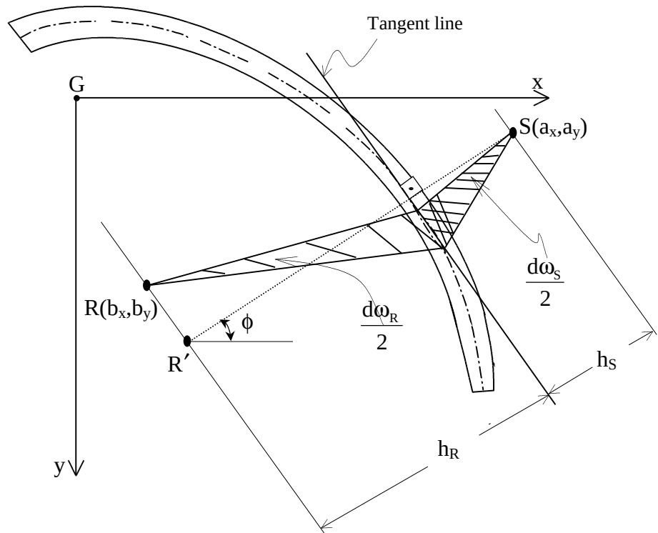
Figure A5.1. Cross-section of a thin-walled beam
