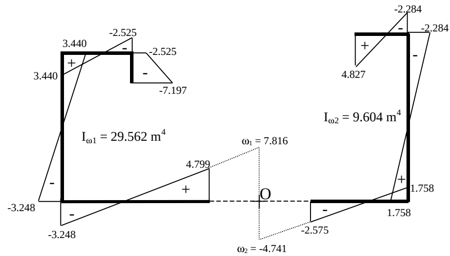
Figure 6.26. The principal sectorial area diagram of the structure in Example 8
