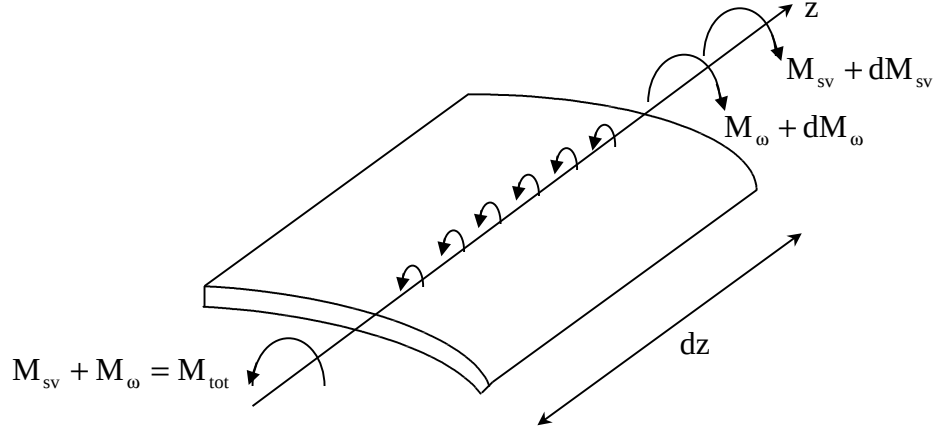
Figure 3.25. Elemental beam loaded by internal and external forces
