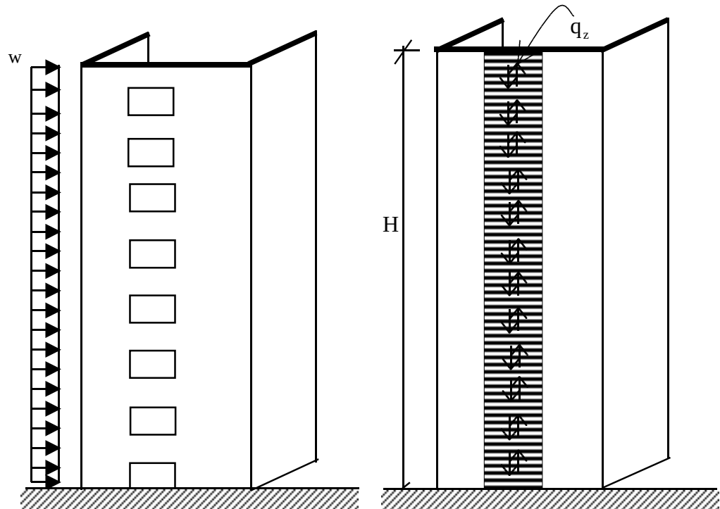
Figure 4.3. (a) Discrete system
