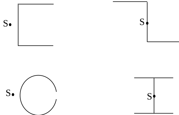
Figure 3.6. Shear centers of typical cross-sectional shapes due to symmetry
