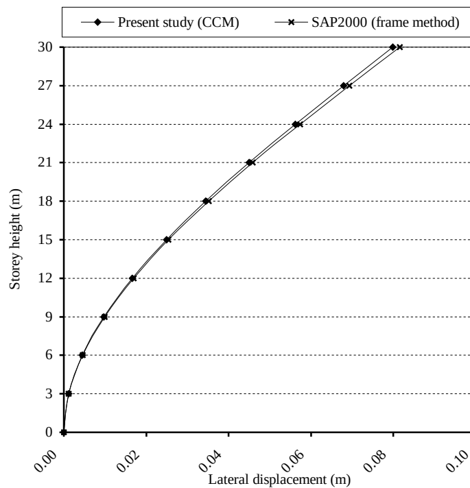
Figure 6.35. The lateral displacements in the X direction in Example 10
