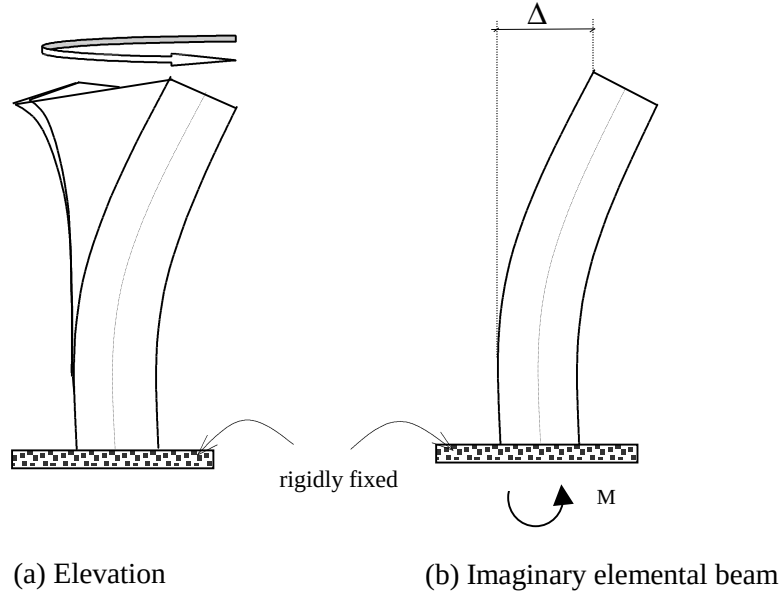
Figure 3.12. Twisting of a rectangular beam (warping restrained)
