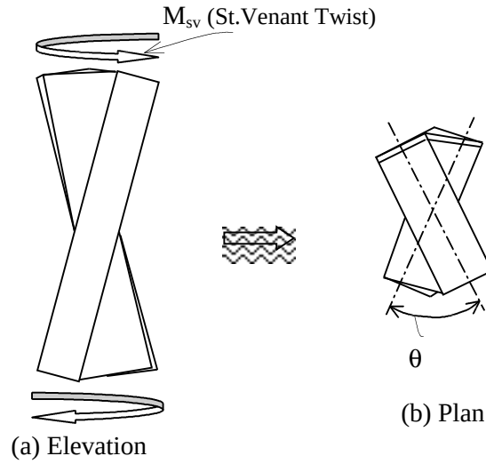
Figure 3.11. Twisting of a rectangular beam (warping not restrained)
