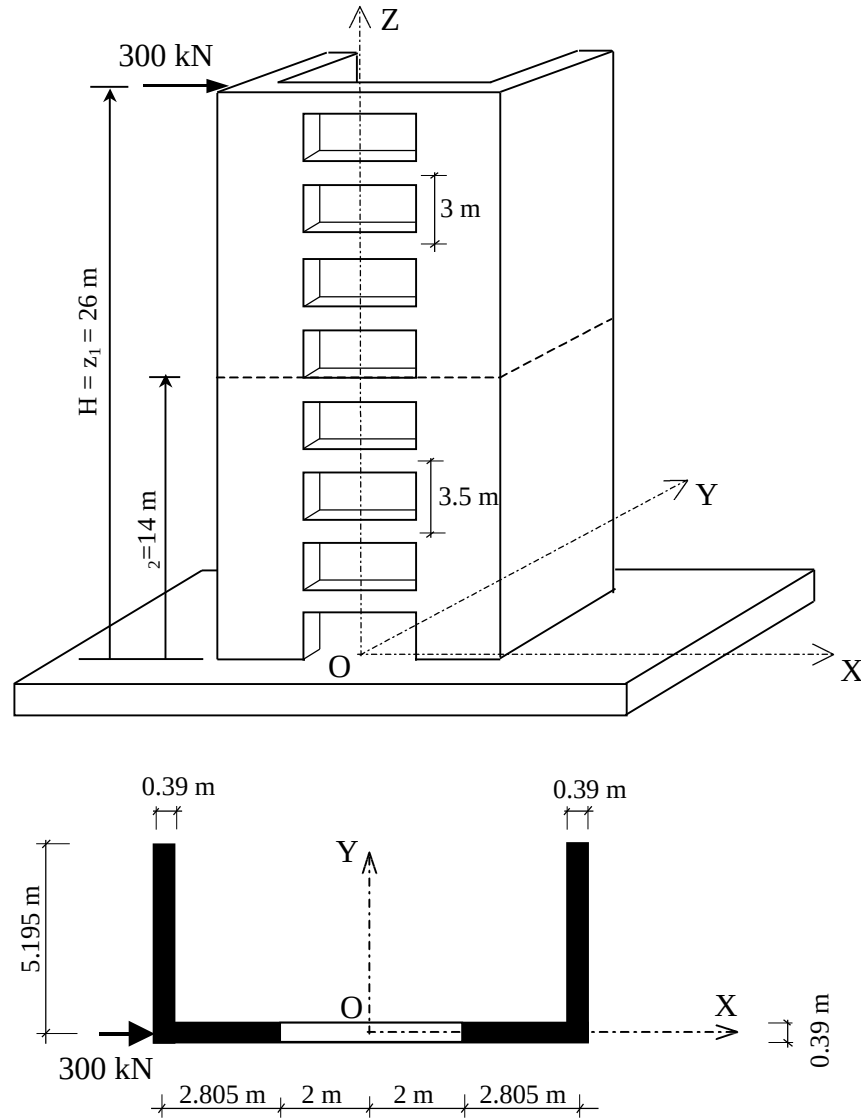
Figure 6.43. Geometrical properties of the structure in Example 12
