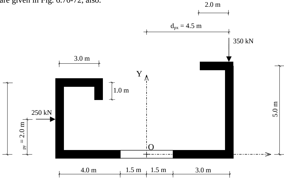
Figure 6.69. Cross-sectional view of the structure in Example 19
