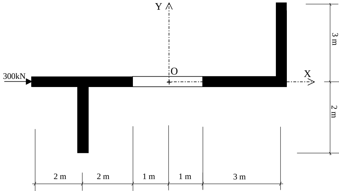
Figure 6.13. Cross-sectional view of the structure in Example 5
