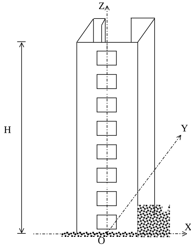
Figure 4.1. Non-planar coupled shear wall
