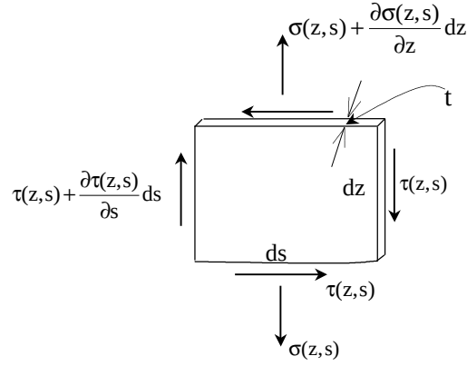
Figure 3.23. Free body diagram of an element ( t \, dz \, ds ) of a thin-walled beam
