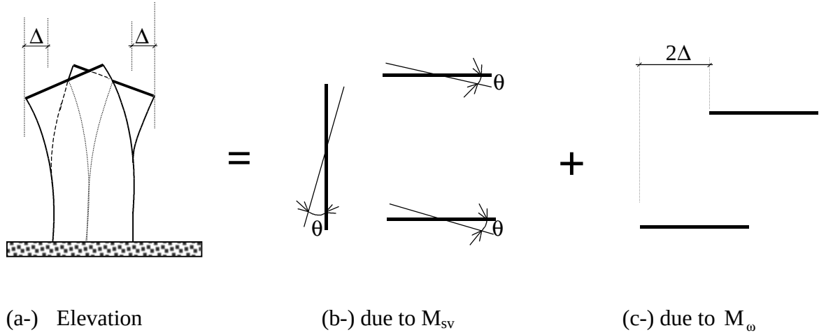
Figure 3.13. A twisting moment and resulting distortions
