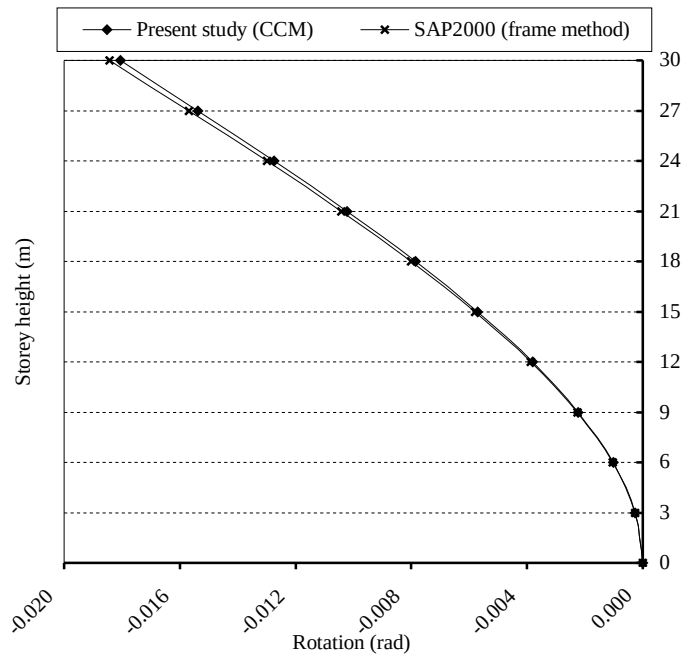
Figure 6.32. The rotations about the Z direction in Example 9
