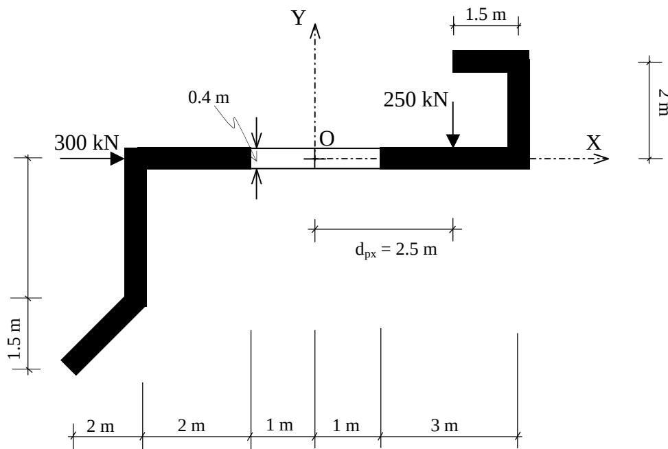
Figure 6.28. Cross-sectional view of the structure in Example 9
