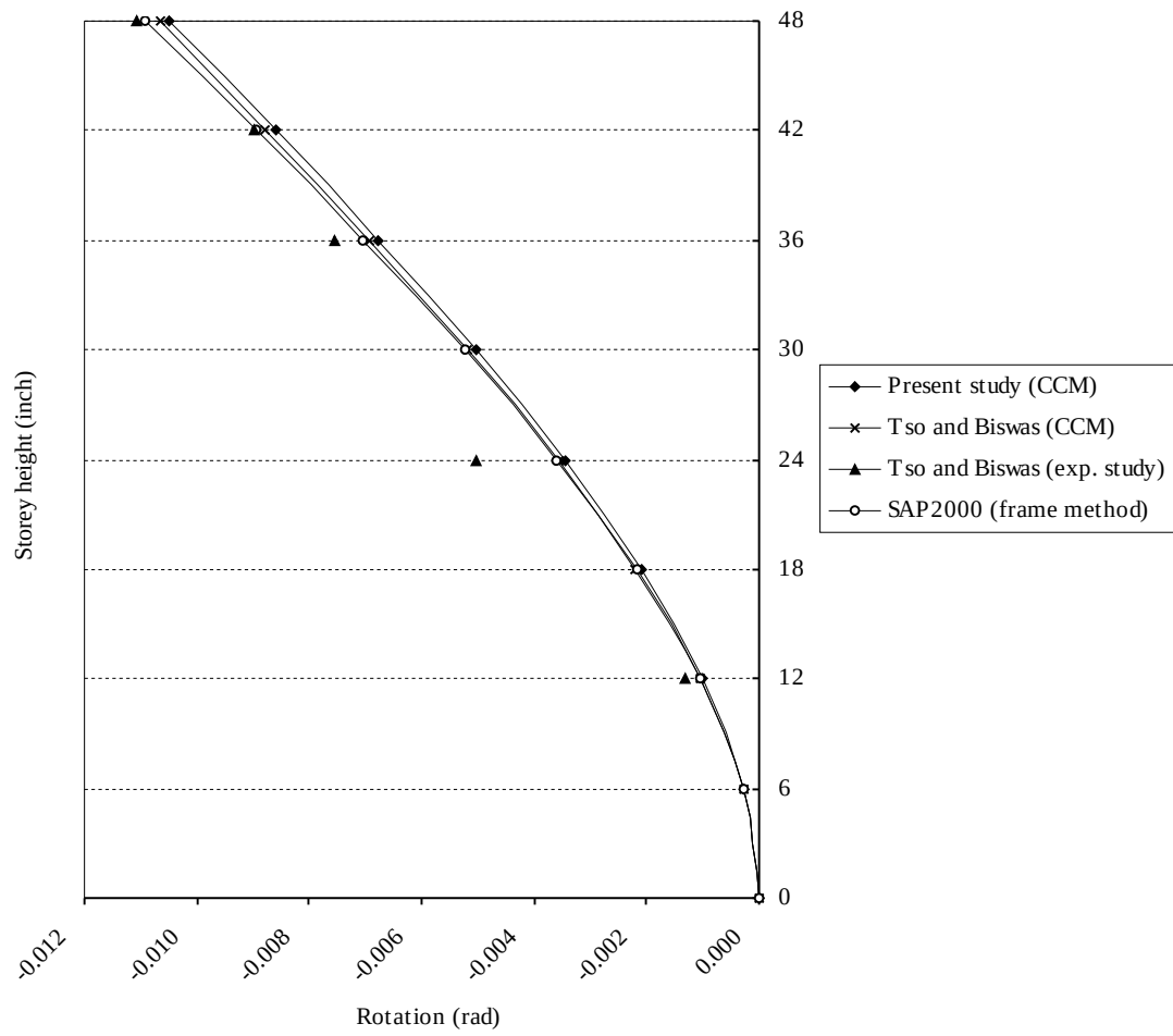
Figure 6.3. The rotations about the Z direction in Example 1
