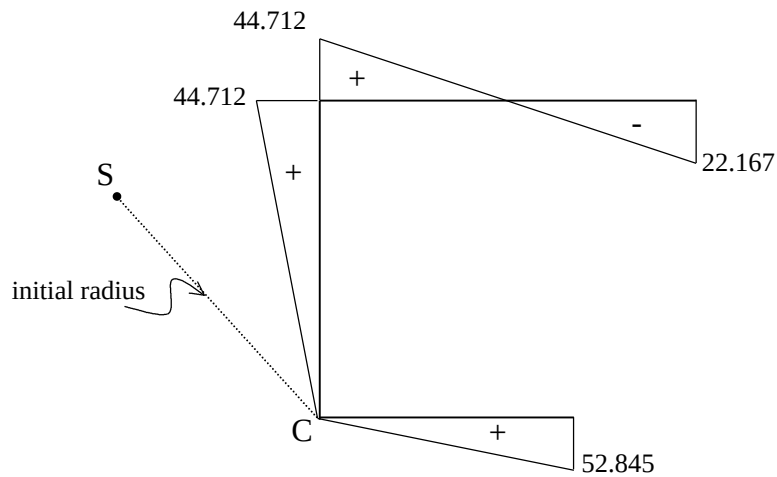
Figure A4.3. Initial sectorial area diagram \omega'
