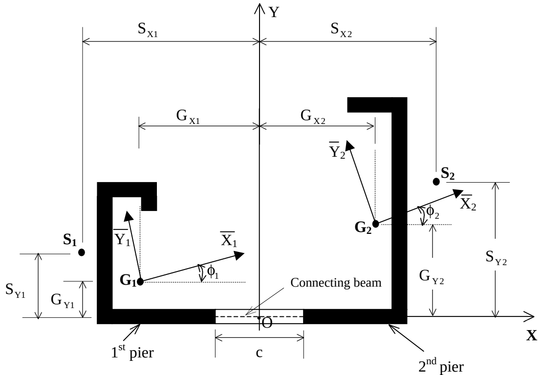
Figure 5.1. Plan of non-planar coupled shear wall
