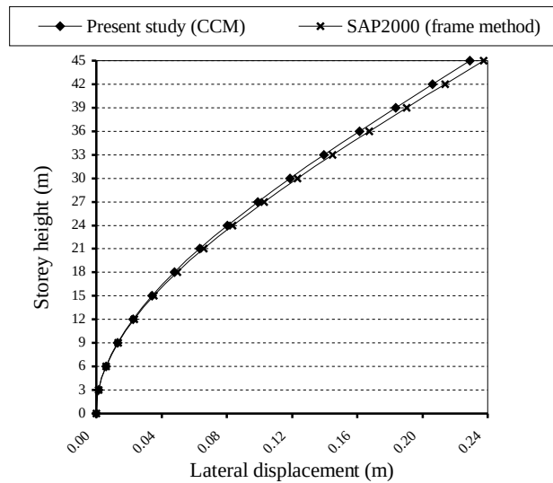
Figure 6.59. The lateral displacements in the X direction in Example16
