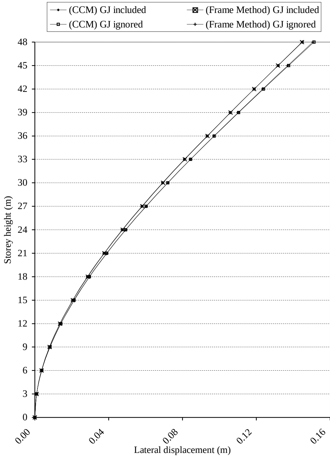
Figure 6.70. The lateral displacements in the X direction in Example 19
