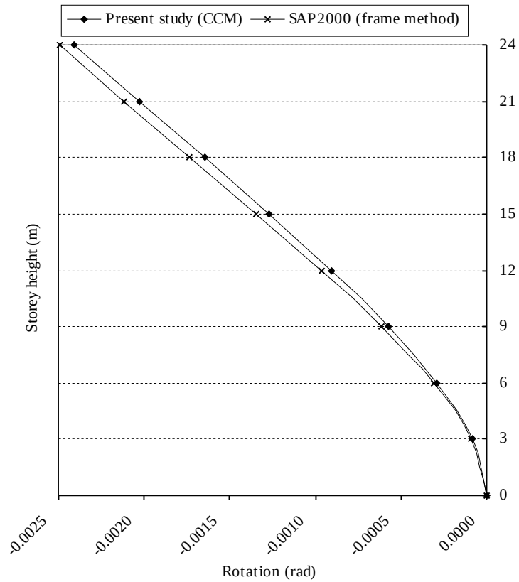
Figure 6.16. The rotations about the Z direction in Example 5
