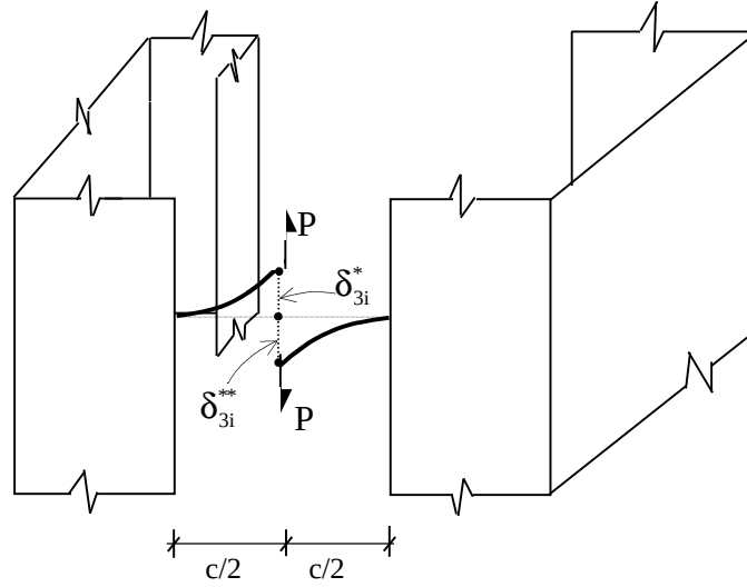
Figure 5.8. Relative displacement of laminae due to bending
