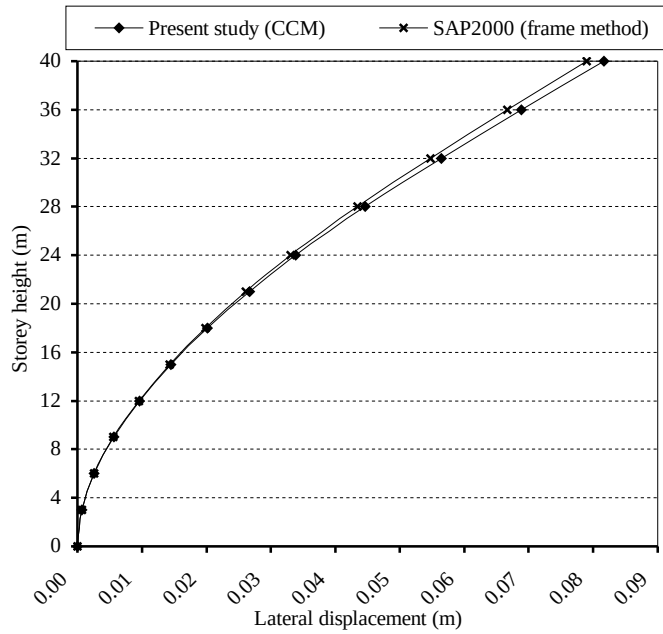
Figure 6.48. The lateral displacements in the X direction in Example 13
