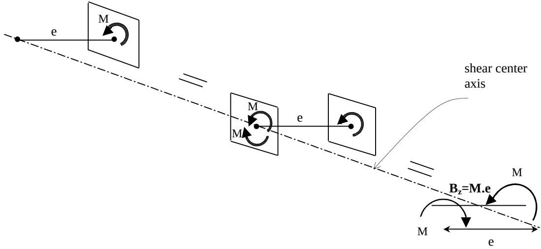
Figure 3.24. Bending moment creating a bimoment
