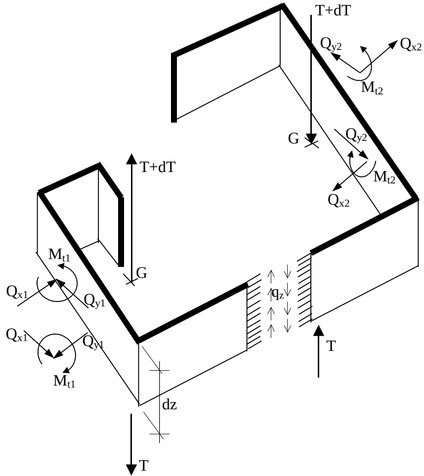
Figure 5.13. Shear forces and torques due to shear flow in connecting medium
