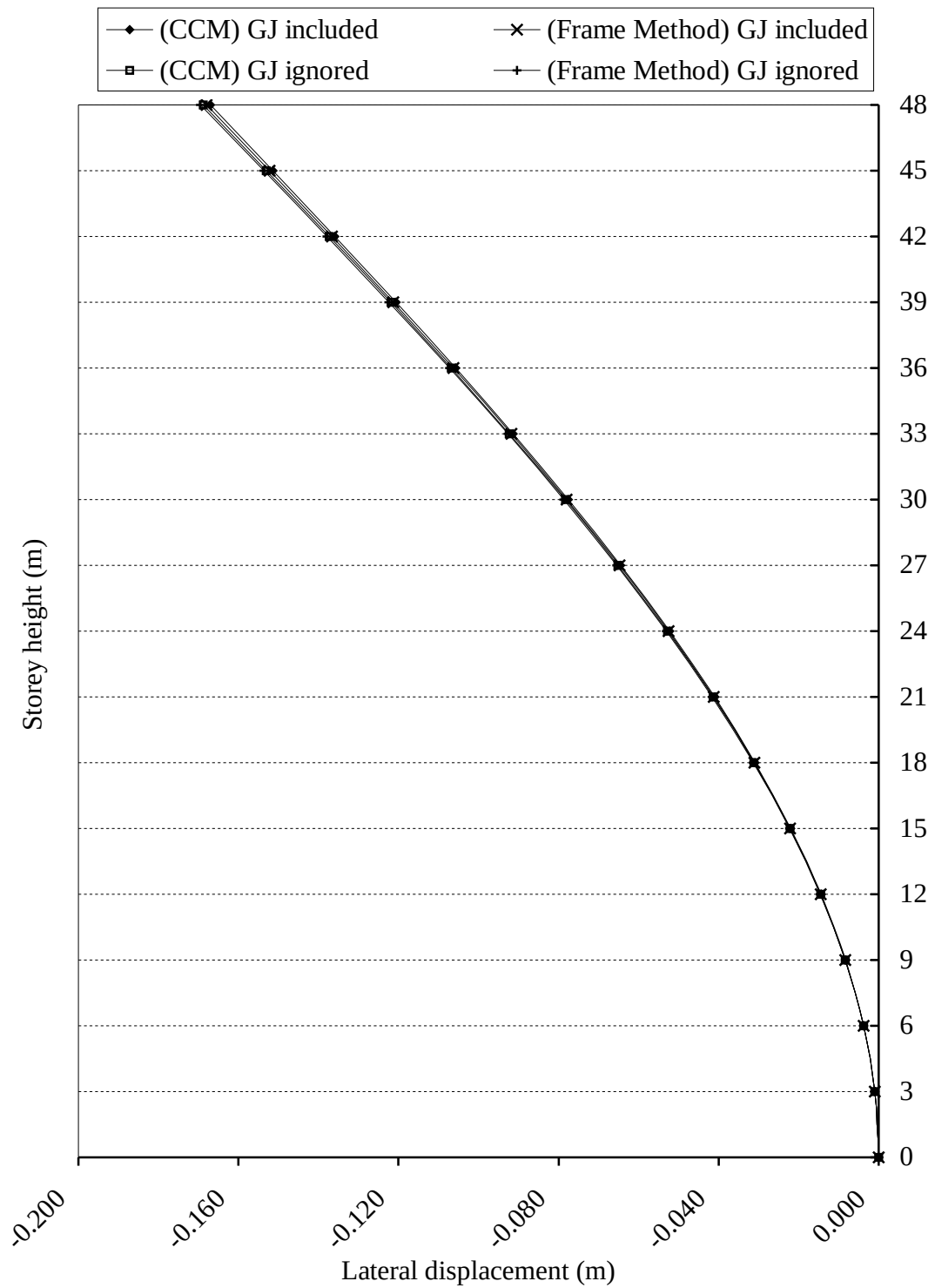
Figure 6.71. The lateral displacements in the Y direction in Example 19
