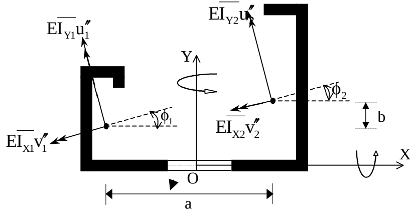
Figure 5.11. Internal moments acting on the components of the coupled shear wall
