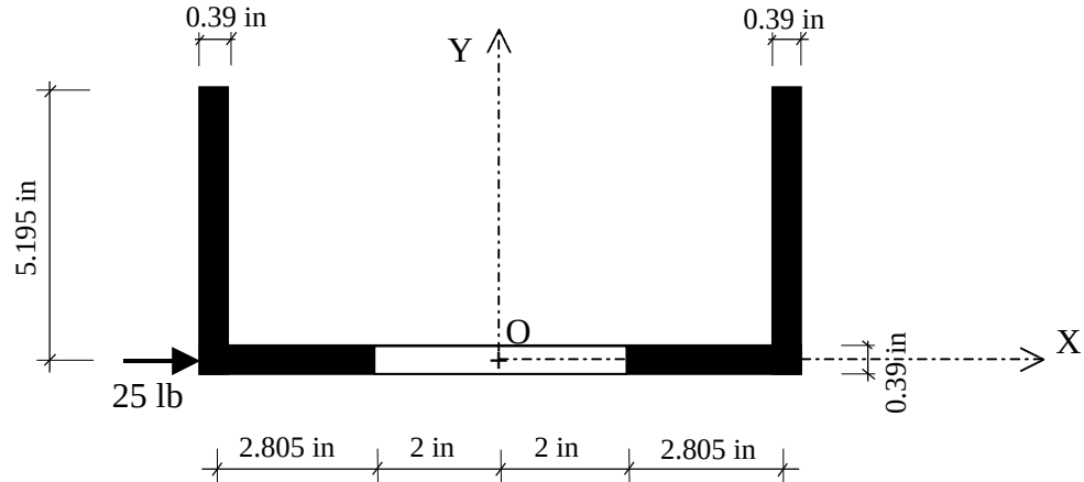
Figure 6.62. Cross-sectional view of the model structure in Example 17
