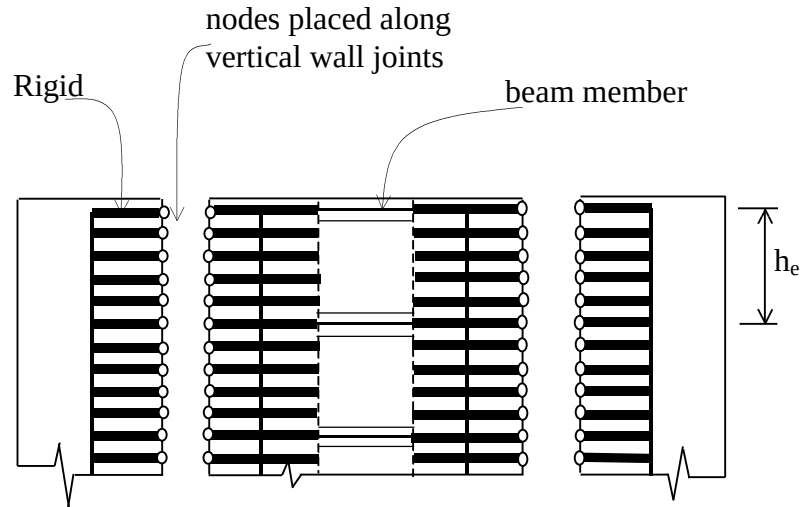
Figure 4.7. Arrangement of wall and beam elements
