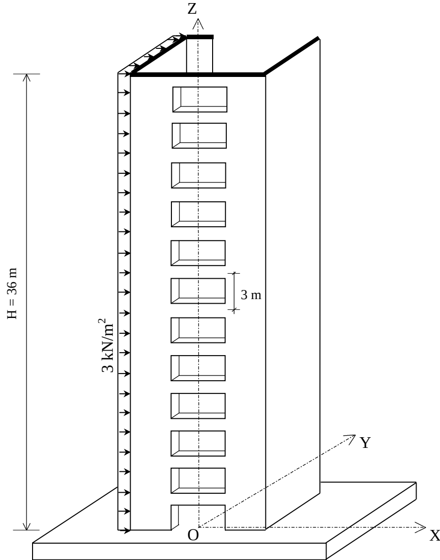
Figure 6.38. Geometrical properties and loading of the structure in Example 11
