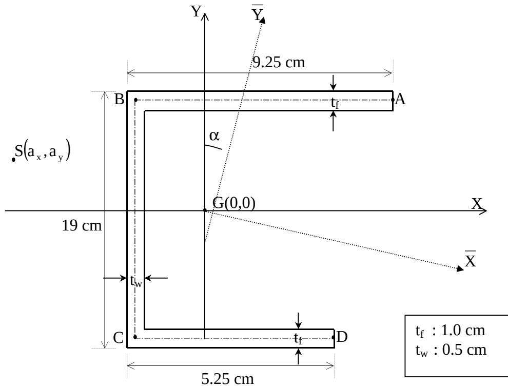
Figure A4.2. Plan of the section
