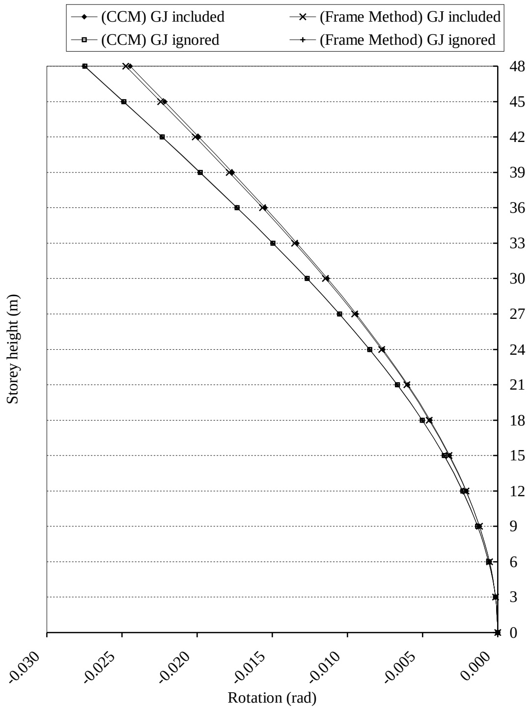
Figure 6.72. The rotations about the Z direction in Example 19
