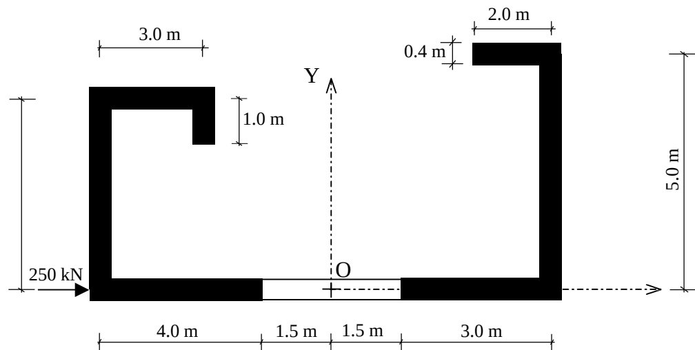
Figure 6.65. Cross-sectional view of the structure in Example 18
