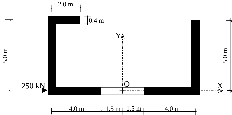
Figure 6.53. Cross-sectional view of the structure in Example 15
