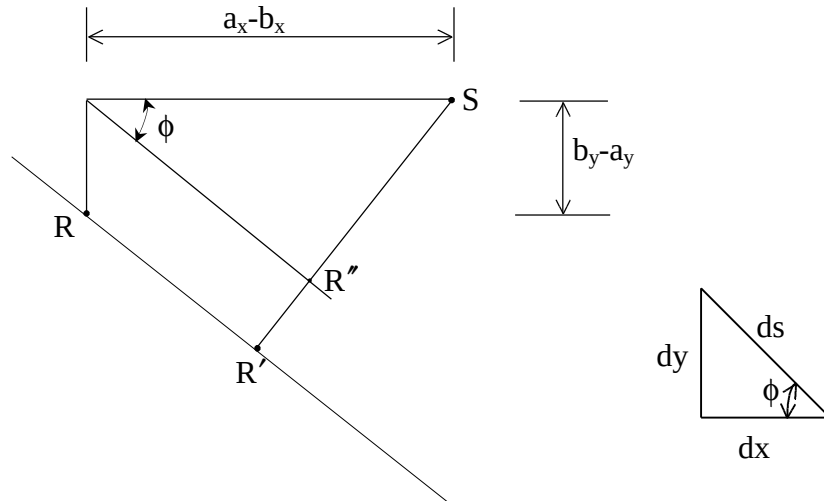
Figure A5.2. Geometric and trigonometric relations in a thin-walled beam
