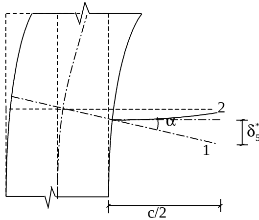
Figure 5.10. Elastic connection condition for connecting beams
