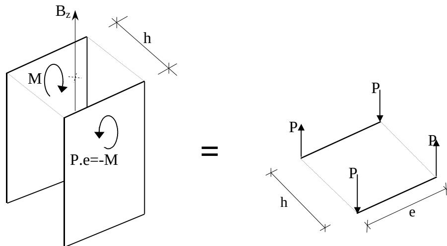
Figure 3.14. Representation of a bimoment
