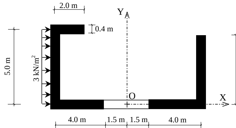
Figure 6.39. Cross-sectional view of the structure in Example 11
