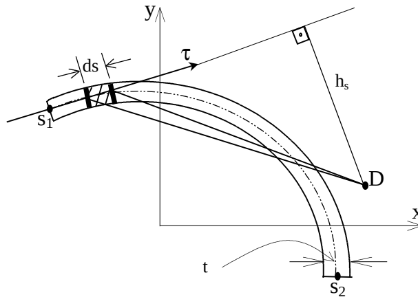
Figure 3.7. Determination of the shear center
