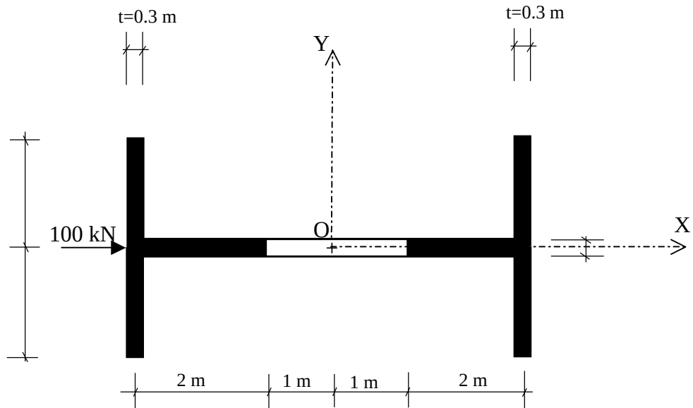
Figure 6.4. Cross-sectional view of the structure in Example 2
