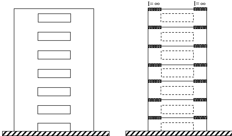
Figure 4.4. Equivalent frame model for planar coupled shear walls
