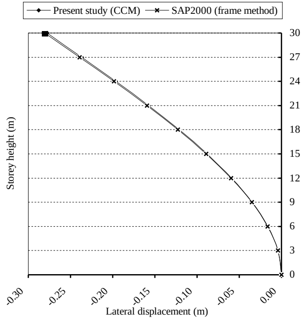
Figure 6.31. The lateral displacements in the Y direction in Example 9
