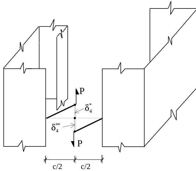
Figure 5.9. Relative displacement of connecting beam due to beam shear deflection
