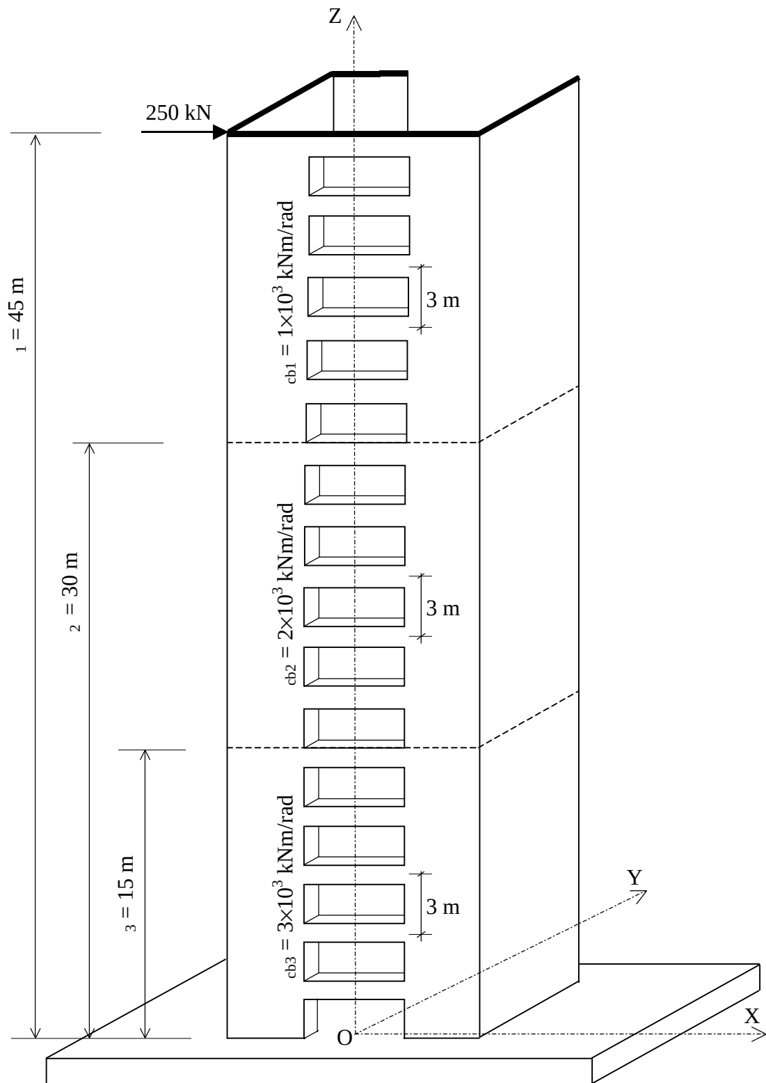
Figure 6.58. Geometrical properties and loading of the structure in Example 16
