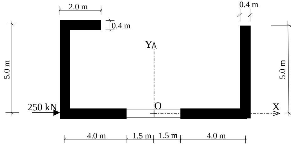
Figure 6.22. Cross-sectional view of the structure in Example 7
