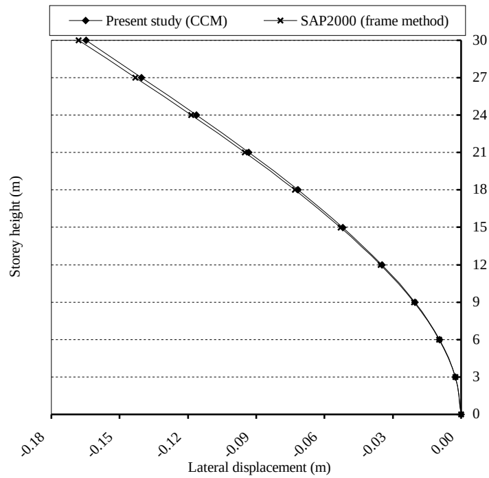
Figure 6.36. The lateral displacements in the Y direction in Example 10
