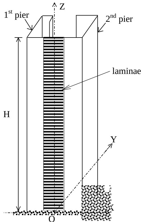
Figure 4.2. Equivalent structure
