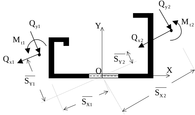
Figure 5.14. Torques and shear forces due to beam shear q_i
