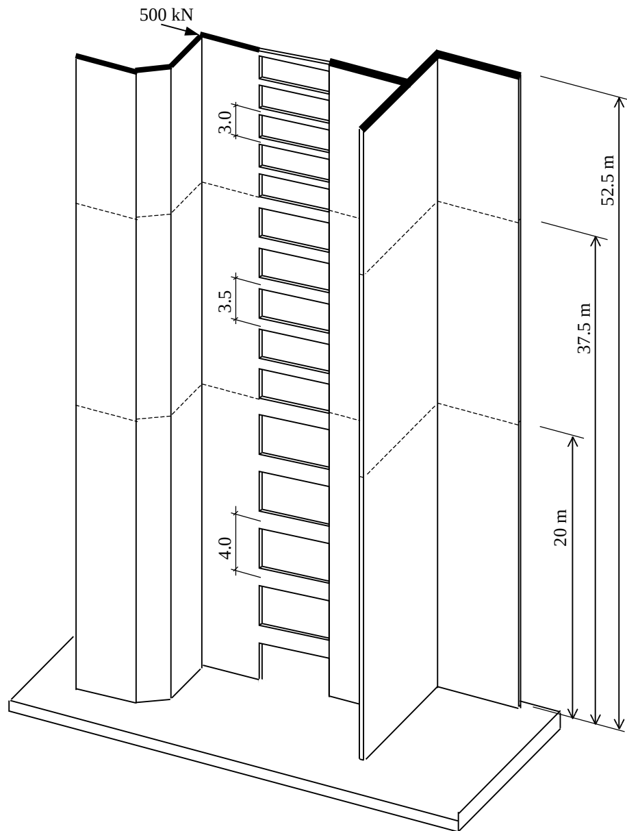
Figure 6.51. Geometric properties and loading of the structure in Example 14
