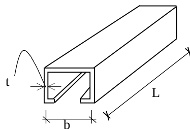
Figure 3.1 Geometrical dimensions of a thin-walled beam
