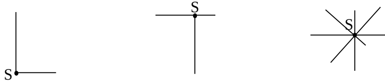
Figure 3.9. Some star sections for which \omega_s = I_{\omega} = 0
