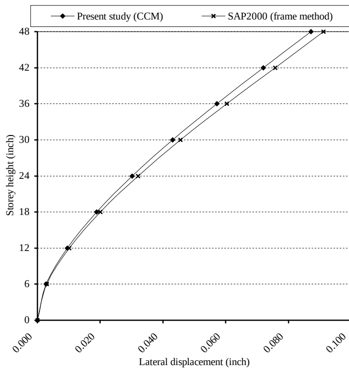
Figure 6.11. The lateral displacements in the X direction in Example 4
