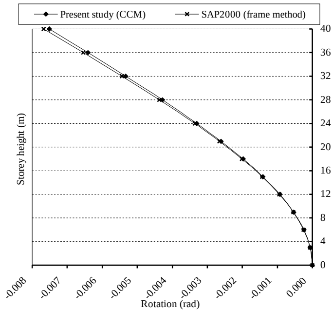
Figure 6.50. The rotations about the Z direction in Example 13
