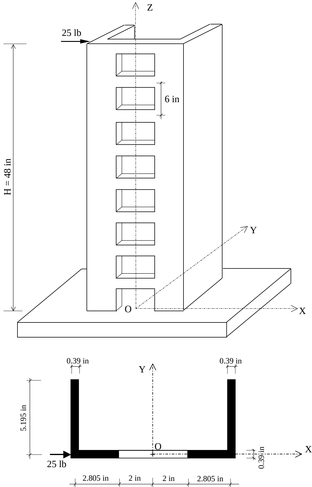
Figure 6.1. Geometrical properties of the model studied by Tso and Biswas
