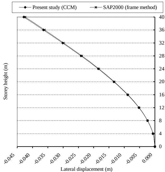
Figure 6.8. The lateral displacements in the Y direction in Example 3
