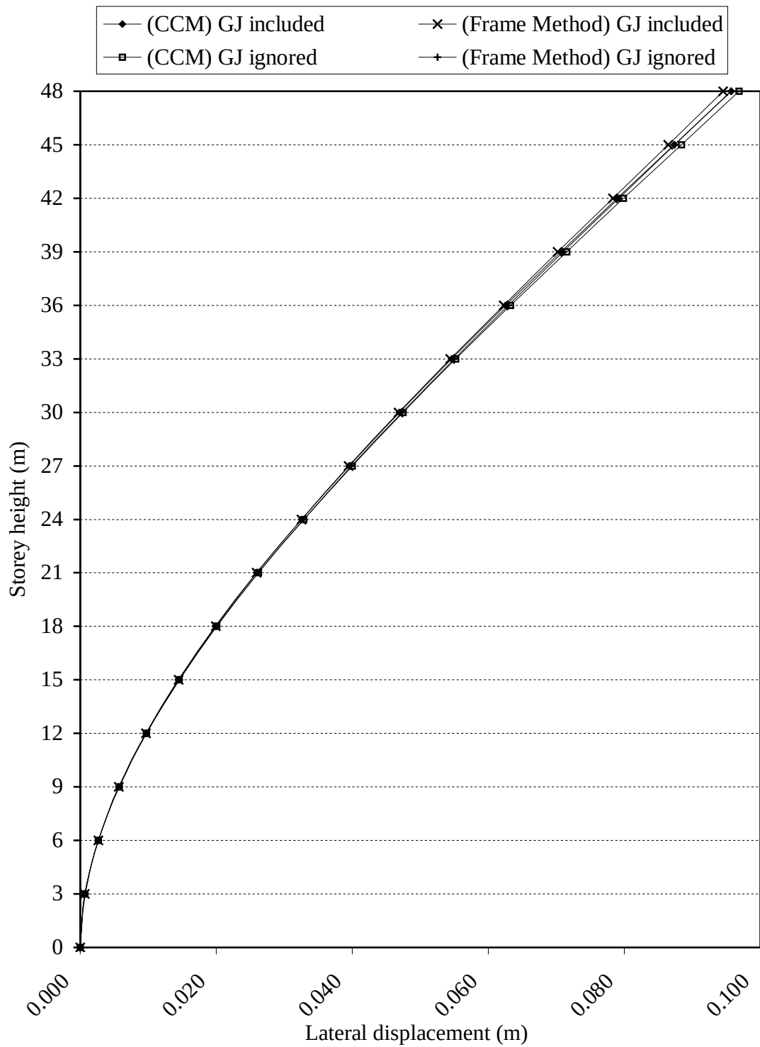
Figure 6.66. The lateral displacements in the X direction in Example 18
