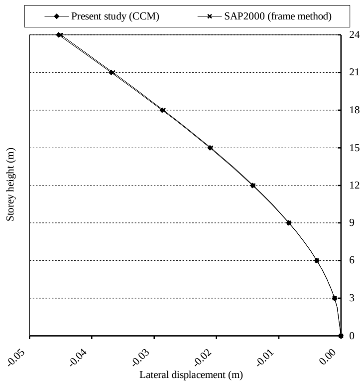
Figure 6.15. The lateral displacements in the Y direction in Example 5
