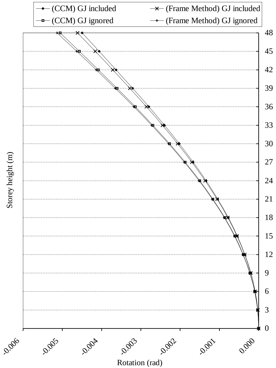
Figure 6.68. The rotations about the Z direction in Example 18
