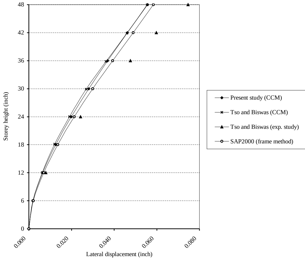
Figure 4.8. The lateral displacements in the X direction of the model studied by Tso& Biswas
