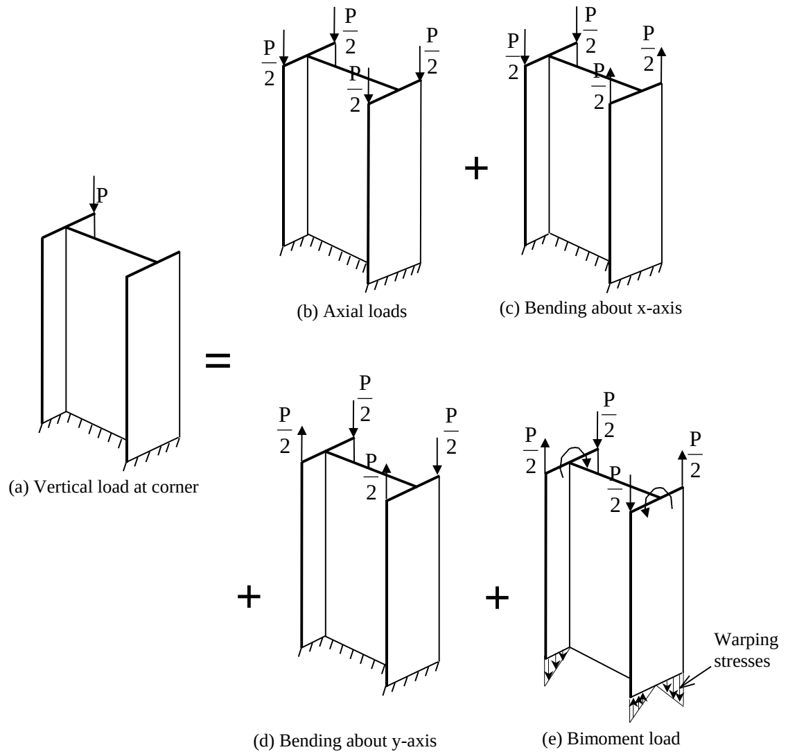
Figure 3.15. A thin-walled I-shaped cantilever column subjected to an eccentric load
