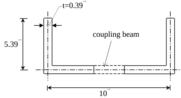
Figure 4.6. Plan of non-planar coupled shear wall tested by Tso and Biswas
