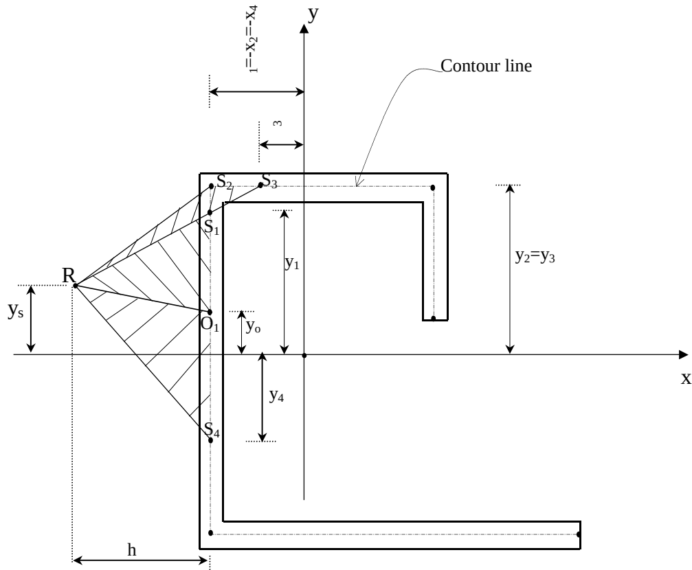
Figure A4.1. Part of the sectorial area diagram for the section
