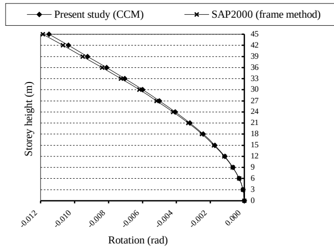
Figure 6.61. The rotations about the Z direction in Example 16
