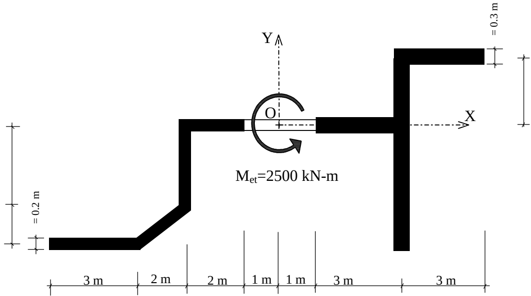
Figure 6.33. Cross-sectional view of the structure in Example 10
