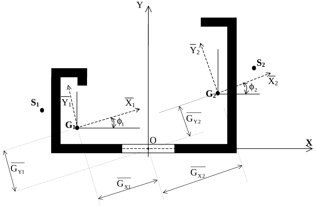
Figure 5.5. Cross-section of a non-planar coupled shear wall
