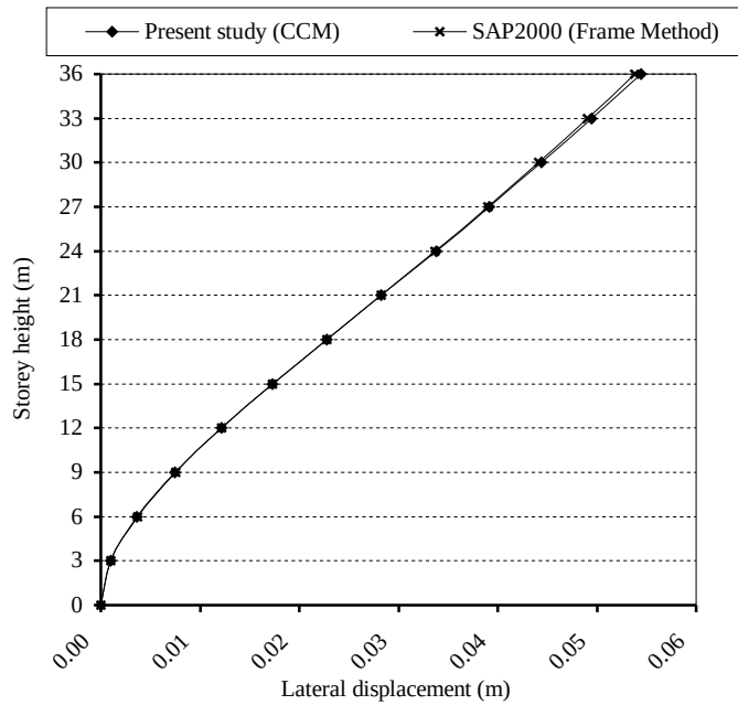
Figure 6.40. The lateral displacements in the X direction in Example 11
