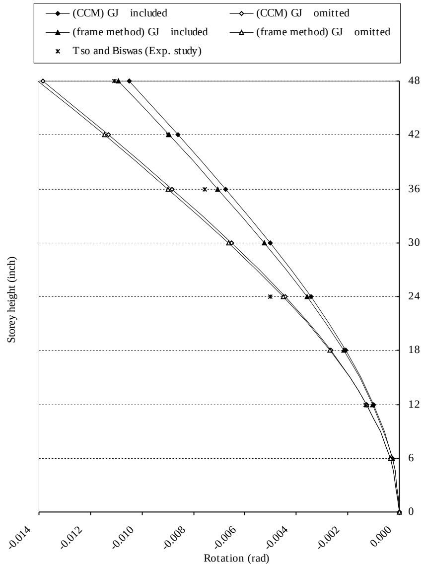
Figure 6.64. The rotations about the Z direction in Example 17
