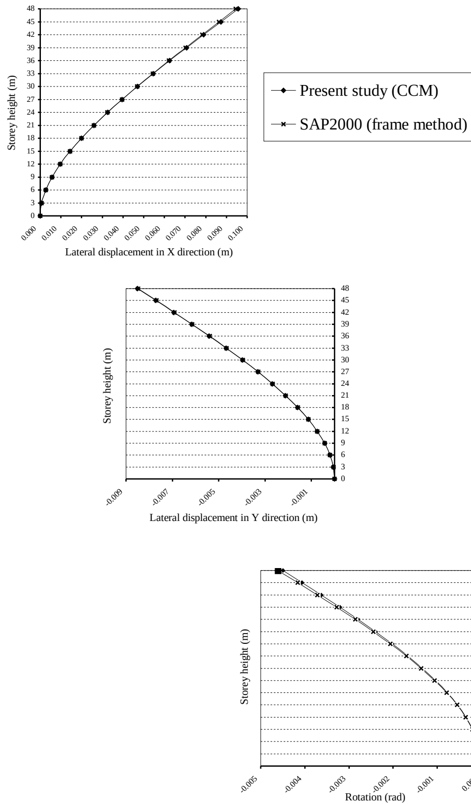
Figure 6.27. The lateral displacements and the rotations along the height in Example 8
