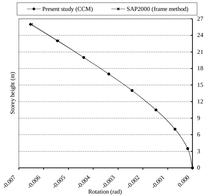
Figure 6.45. The rotations about the Z direction in Example 12
