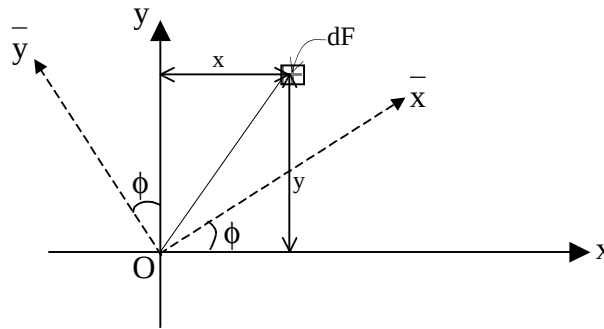
Figure 5.2. Rotation of axes
