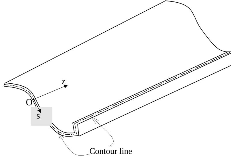
Figure 3.3. General form of an open bar
