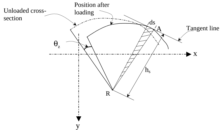
Figure 3.21. Displacement of a section in non-uniform torsion
