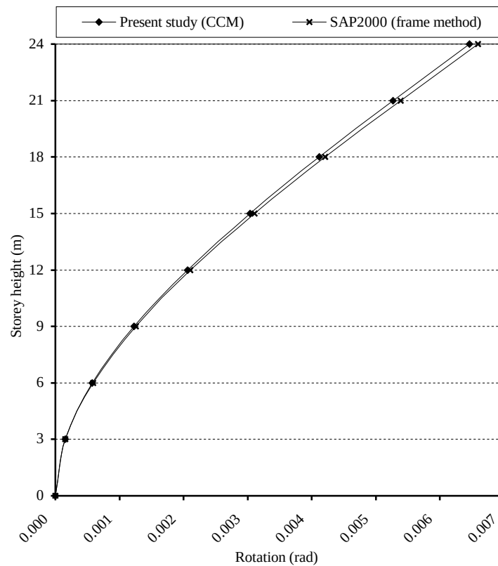
Figure 6.21. The rotations about the Z direction in Example 6
