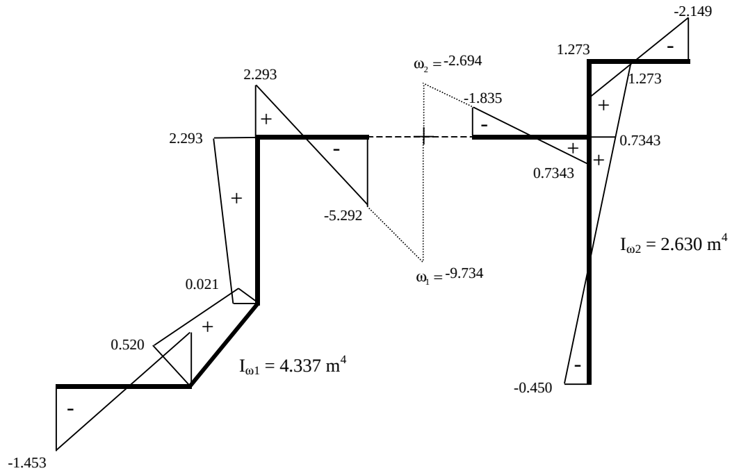
Figure 6.34. The principal sectorial area diagram of the structure in Example 10
