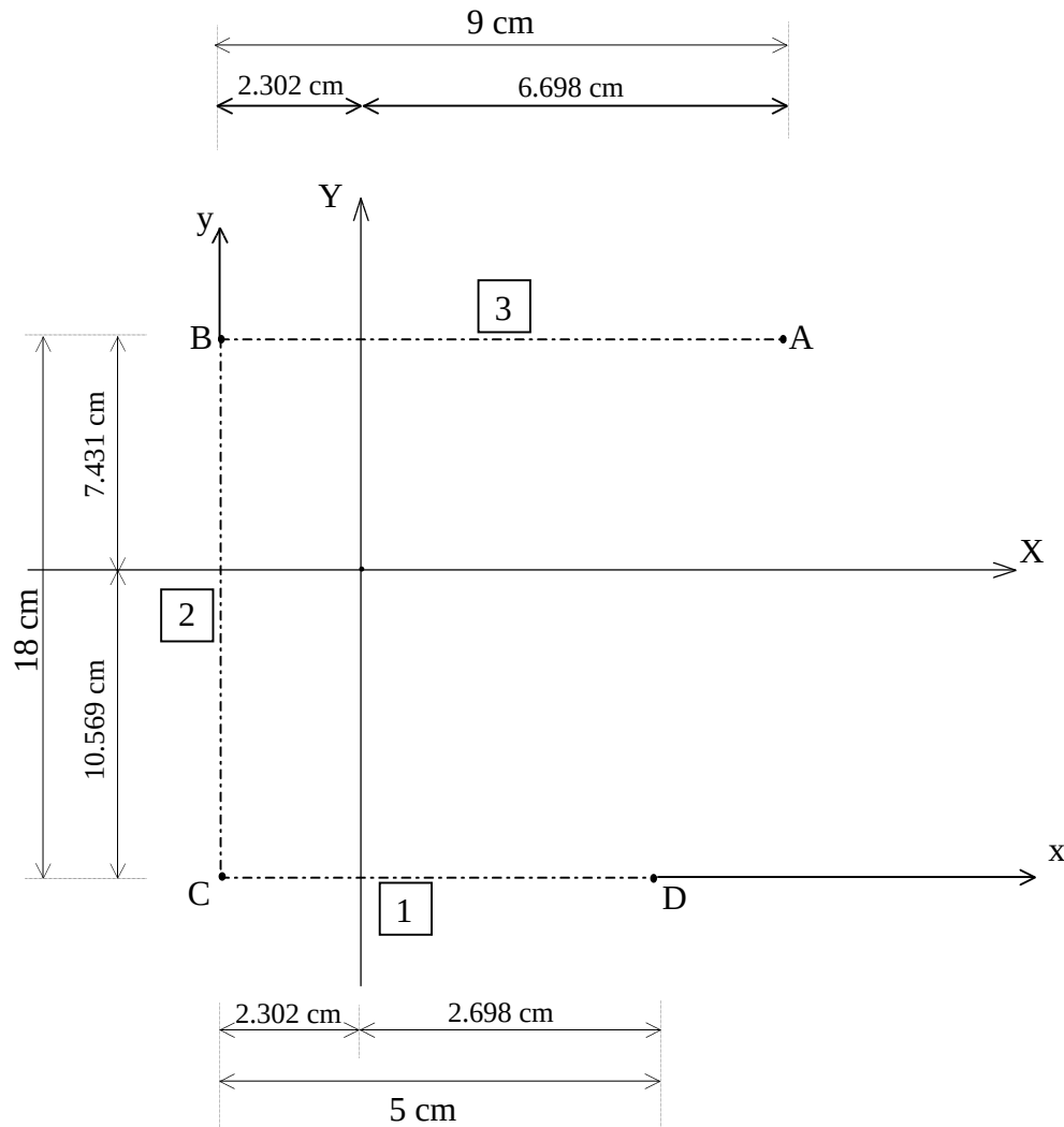
Figure A4.3. Contour of the section
