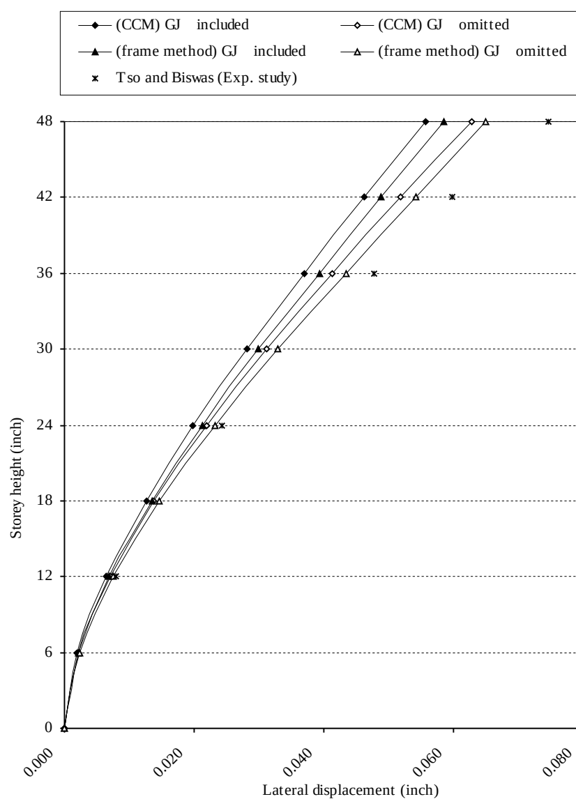
Figure 6.63. The lateral displacements in the X direction in Example 17
