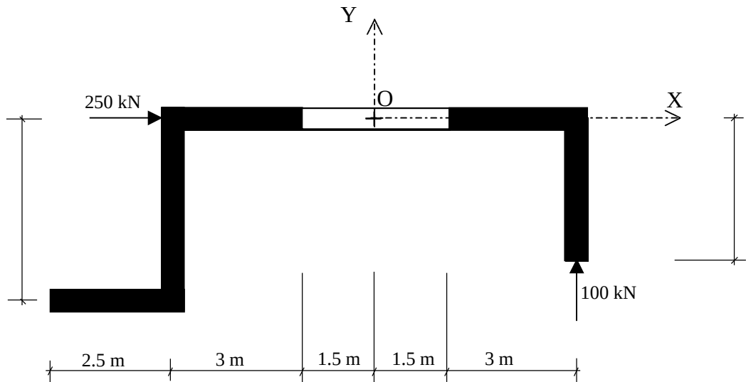
Figure 6.17. Cross-sectional view of the structure in Example 6
