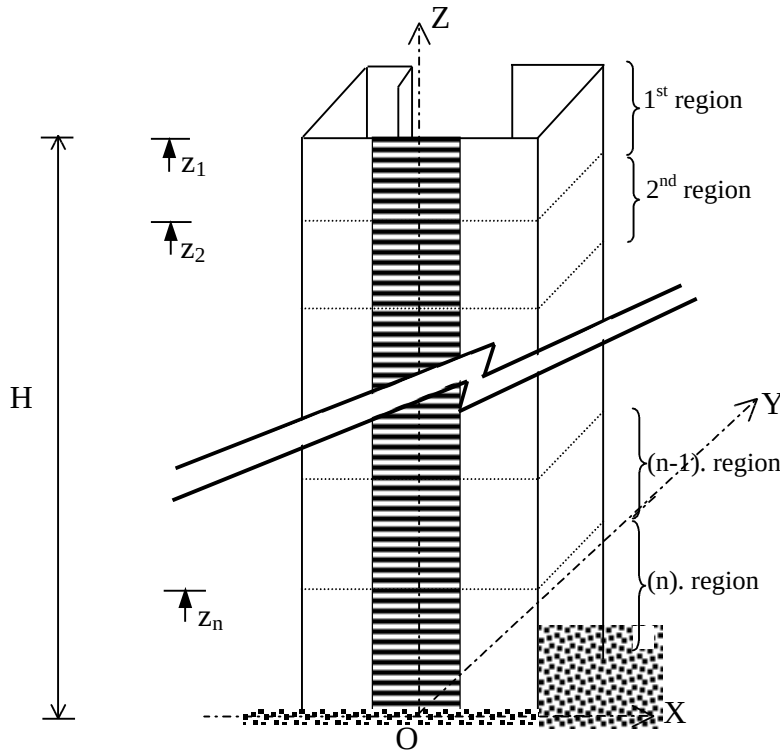
Figure 5.3. Equivalent structure
