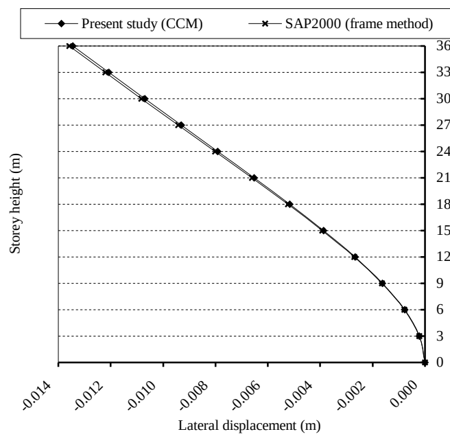
Figure 6.41. The lateral displacements in the Y direction in Example 11
