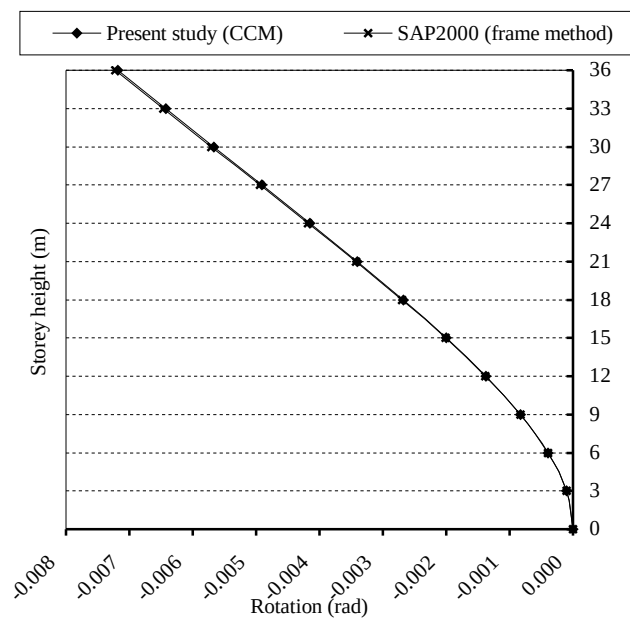
Figure 6.42. The rotations about the Z direction in Example 11
