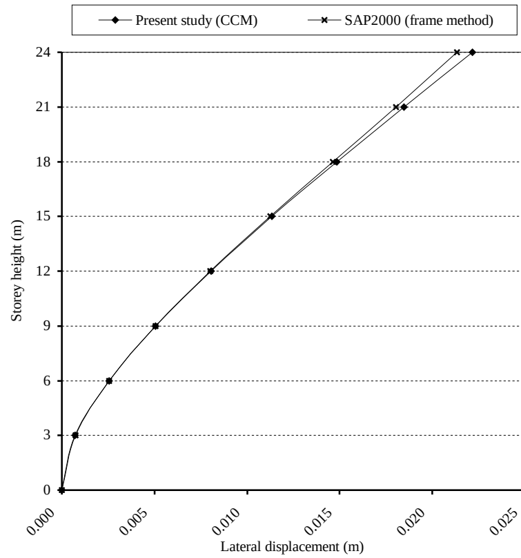
Figure 6.5. The lateral displacements in the X direction in Example 2
