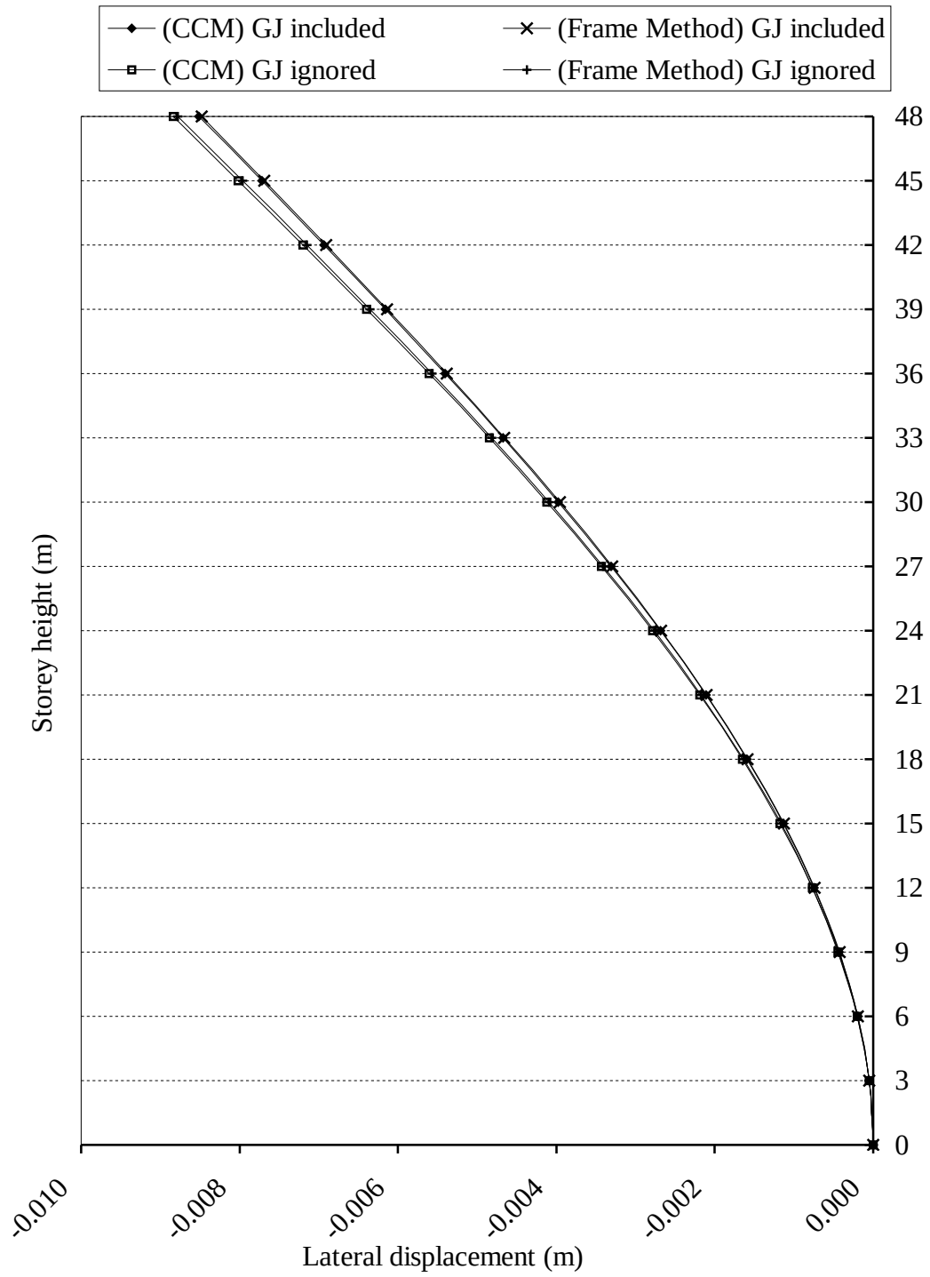
Figure 6.67. The lateral displacements in the Y direction in Example 18
