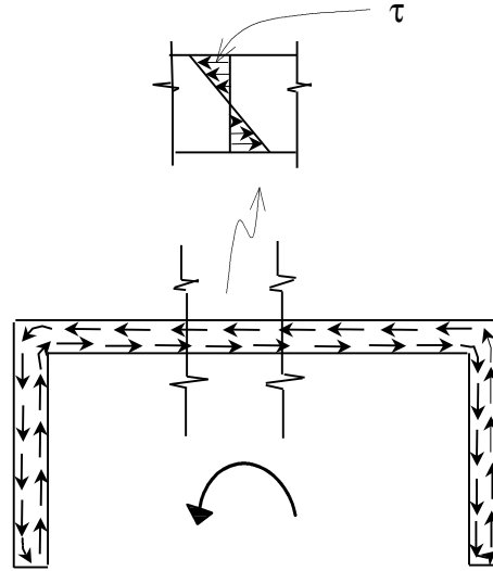
Figure 3.4. Stress distribution in a twisted open section beam
