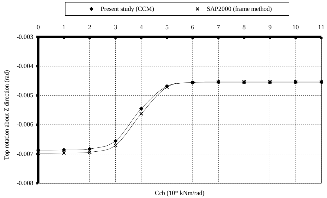
Figure 6.56. The effect of the variation of the connection stiffness on the maximum top rotation about the Z direction in example 15
