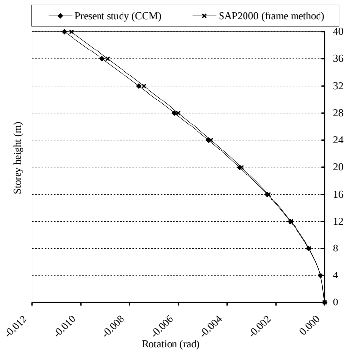
Figure 6.9. The rotations about the Z direction in Example 3
