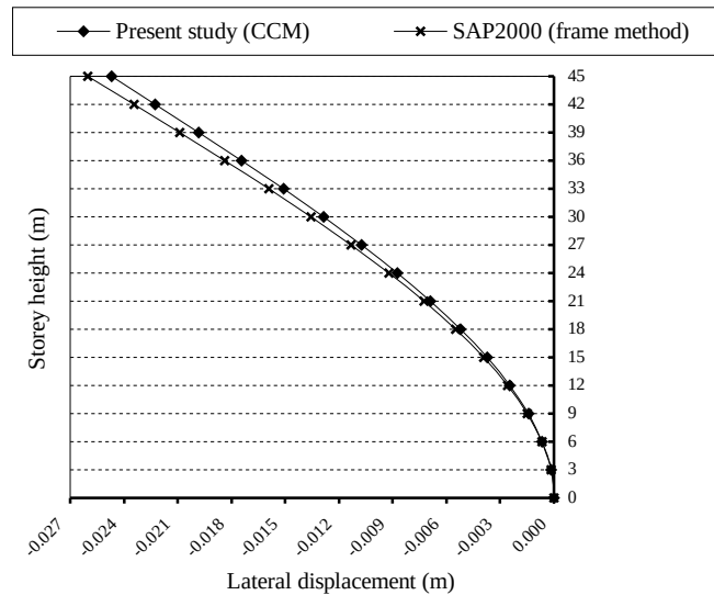
Figure 6.60. The lateral displacements in the Y direction in Example 16
