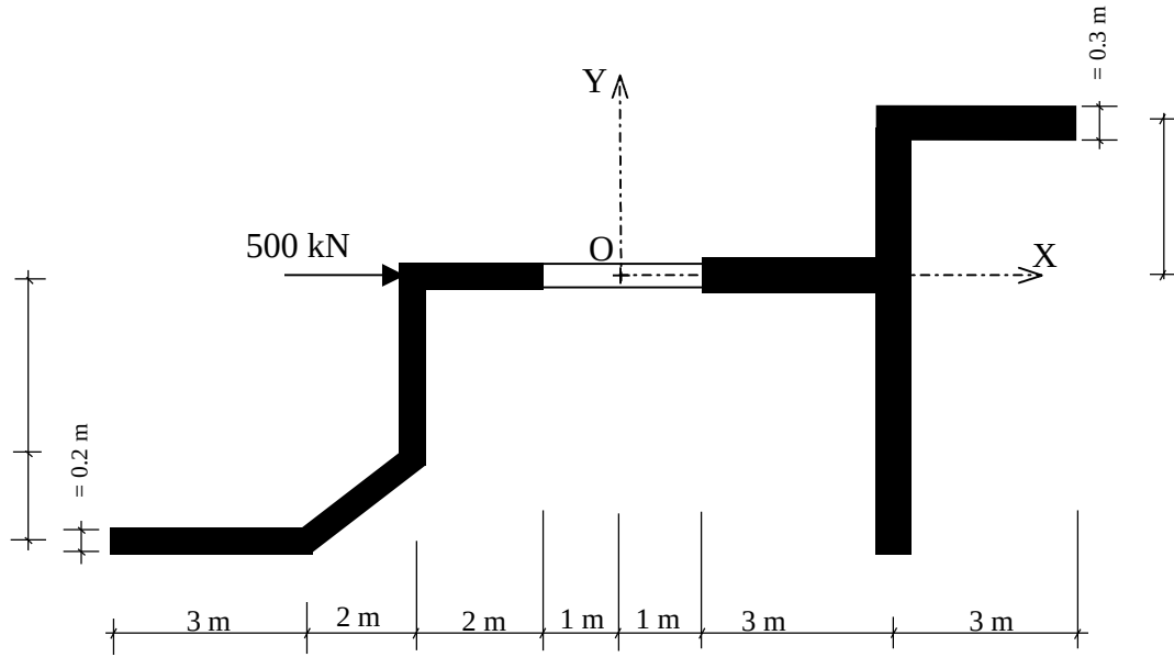
Figure 6.52. Cross-sectional view of the structure in Example 14
