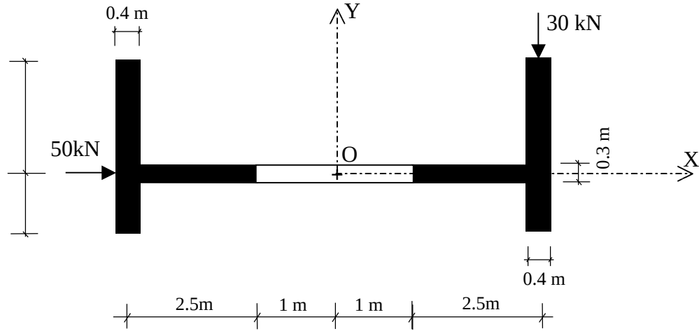
Figure 6.6. Cross-sectional view of the structure in Example 3
