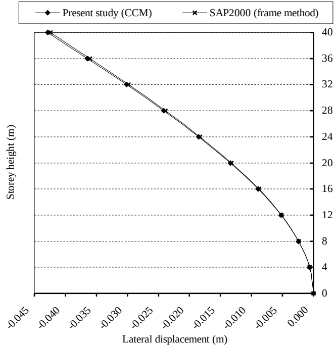
Figure 6.7. The lateral displacements in the X direction in Example 3
