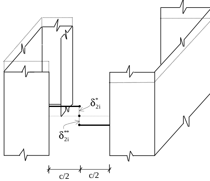
Figure 5.7. Relative displacements due to axial forces in the piers
