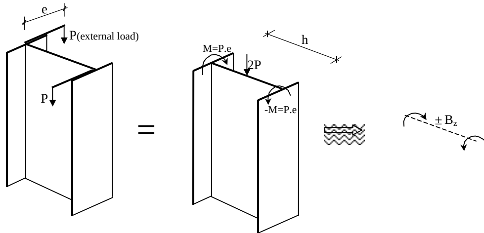
Figure 3.17. Bimoment creating a twist
