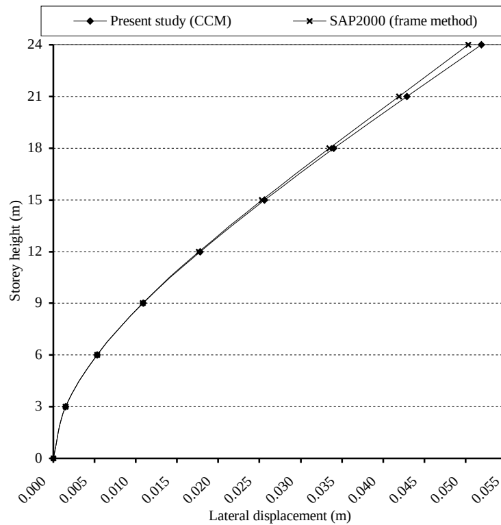
Figure 6.14. The lateral displacements in the X direction in Example 5
