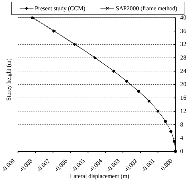
Figure 6.49. The lateral displacements in the Y direction in Example 13
