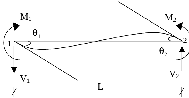
Figure 5.4. General displacement of a connecting beam
