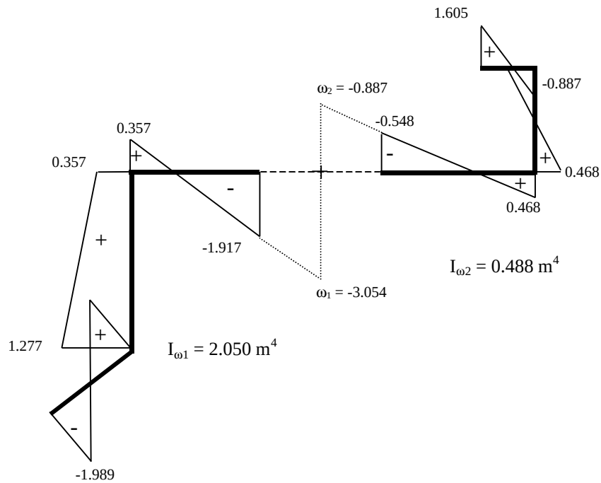
Figure 6.29. The principal sectorial area diagram of the structure in Example 9
